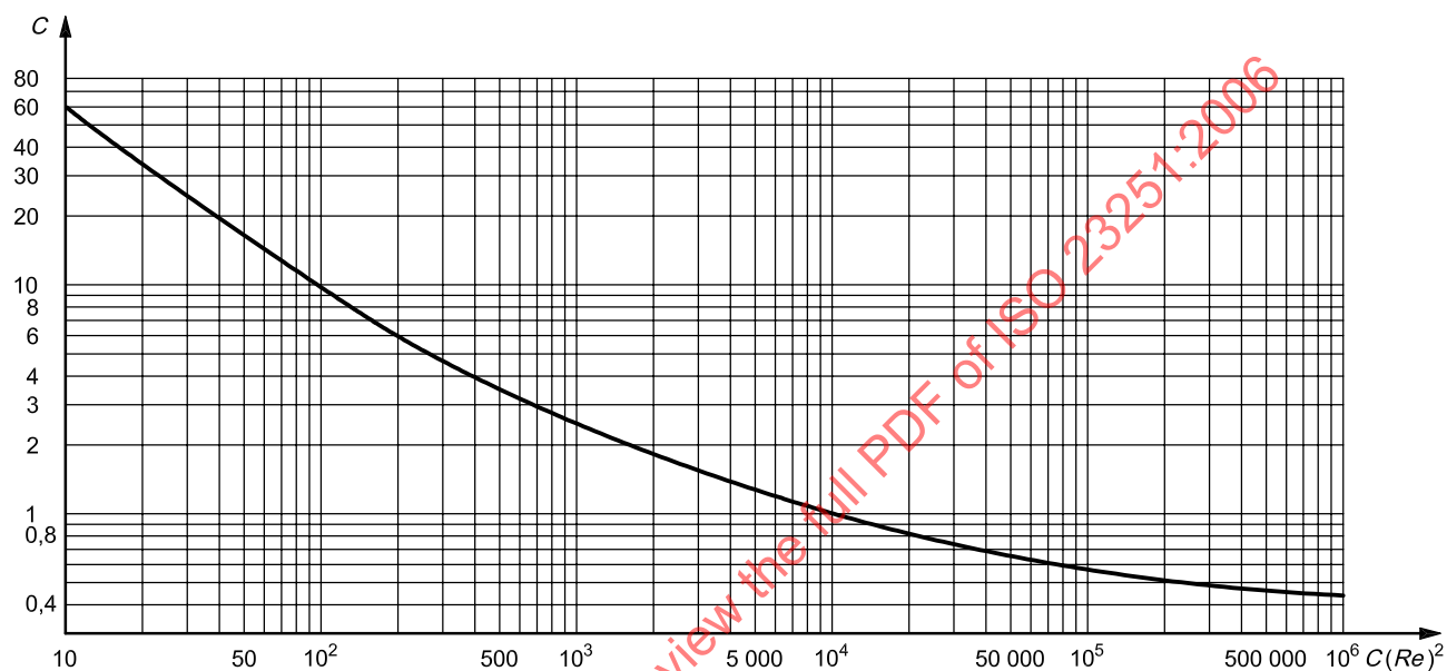
Figure 16 — Determination of drag coefficient
