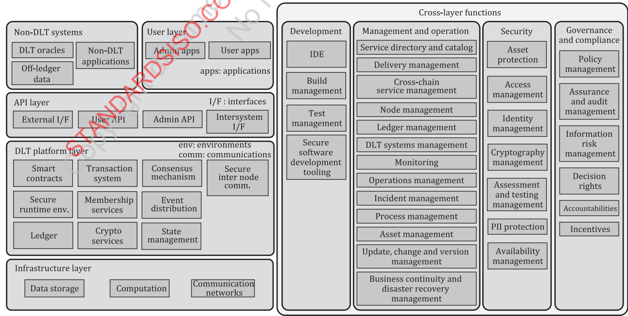
Figure 8 — Functional components
