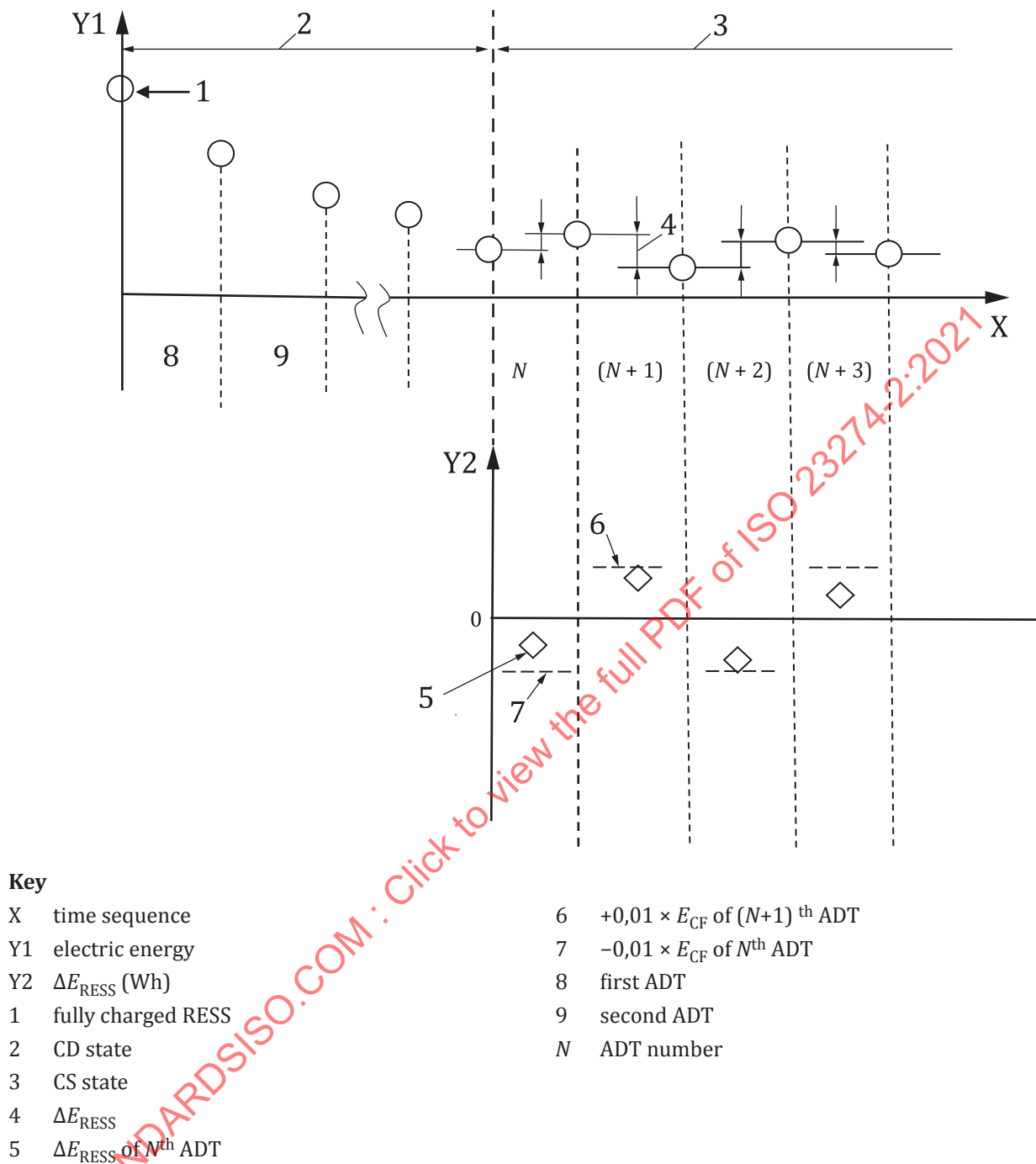
Figure 1 — Determination of transition point from CD to CS state (case 1)
