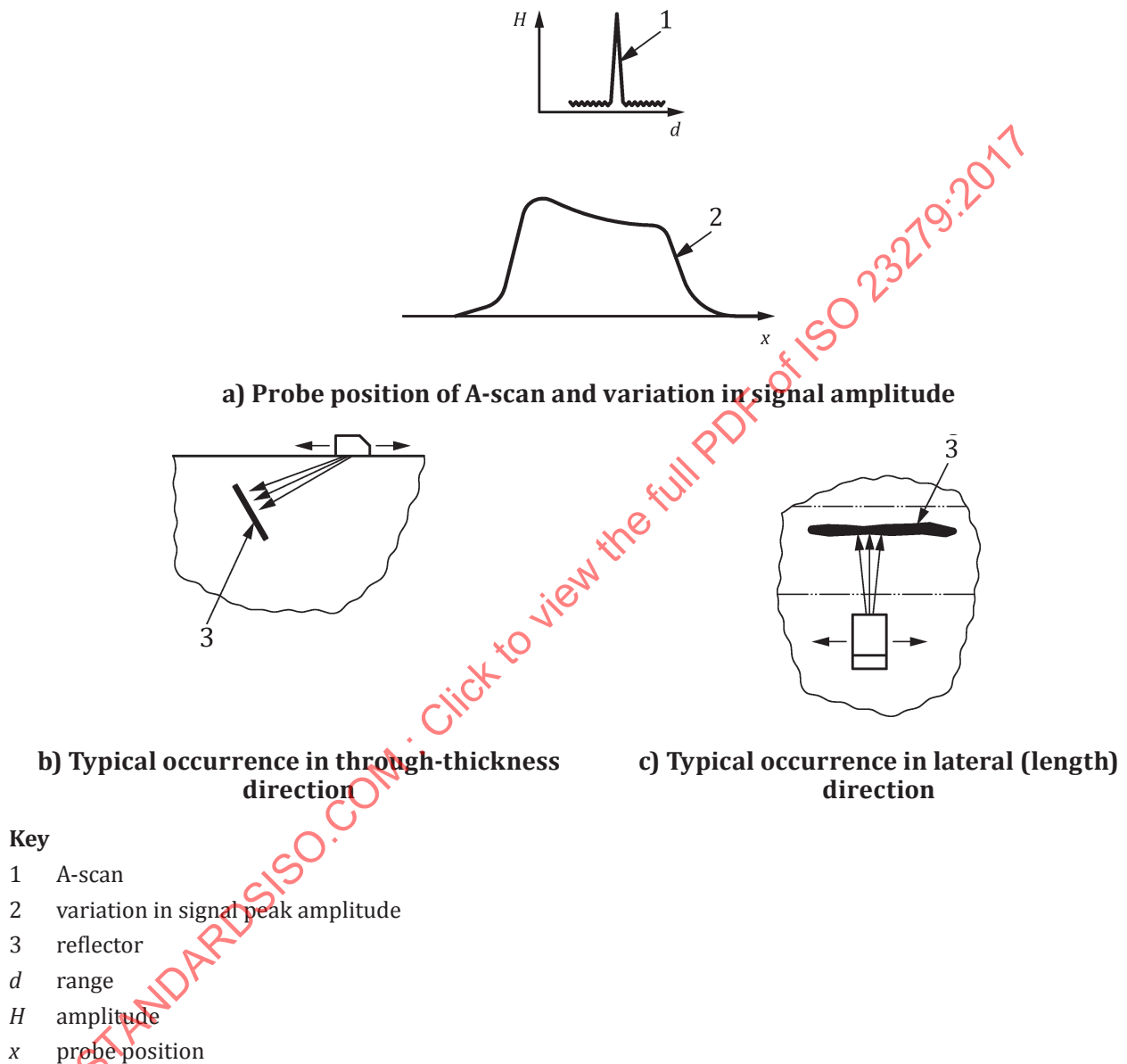
Figure C.2 — Pattern 2 ultrasonic response
