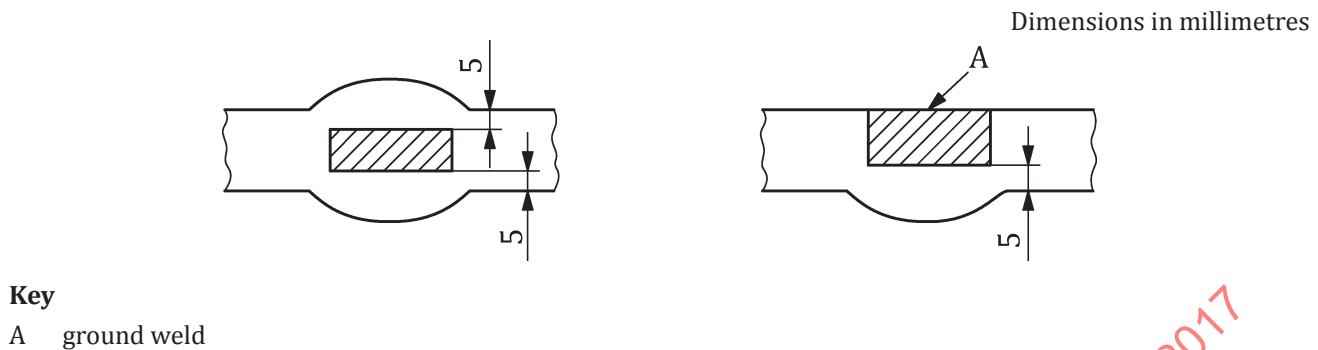
Figure 1 — Origin of indications from a weld
