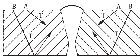
a) Transverse waves, T
