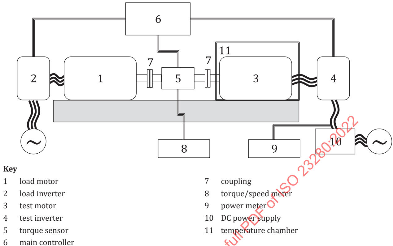
Figure 3 — Schematic diagram of the test system
