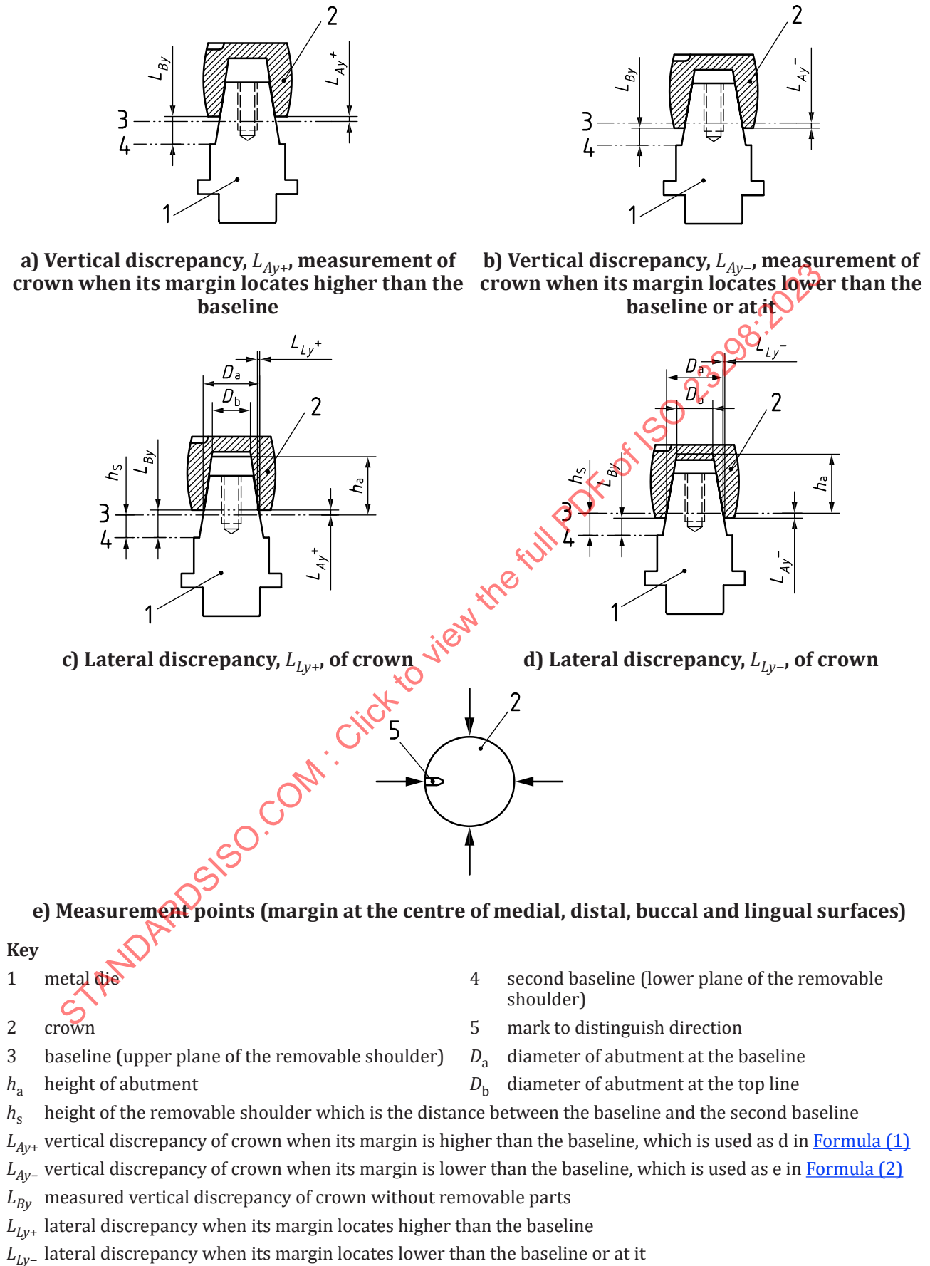
Figure 6 — Discrepancy measurement of the crown
