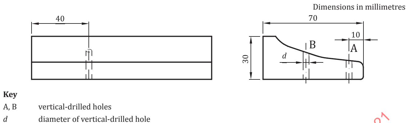
Figure J.4 — Typical reference block for angle-beam probe technique on foot toe and ankle
