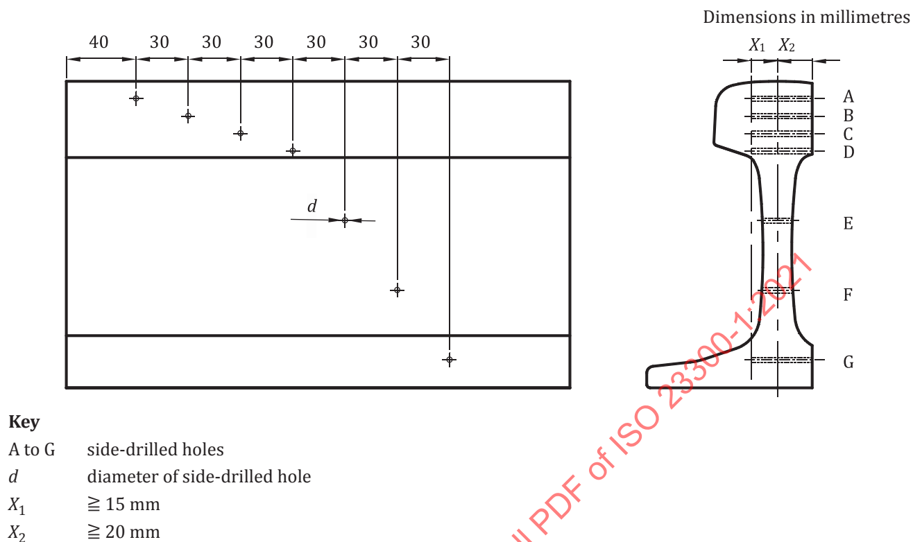
Figure J.2 — Typical reference block for normal-beam probe technique
