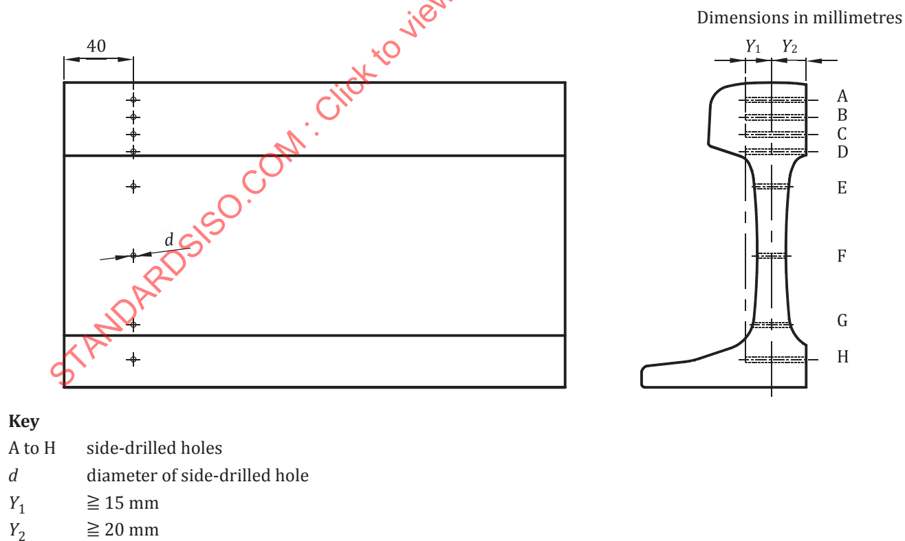
Figure J.3 — Typical reference block for angle-beam probe technique
