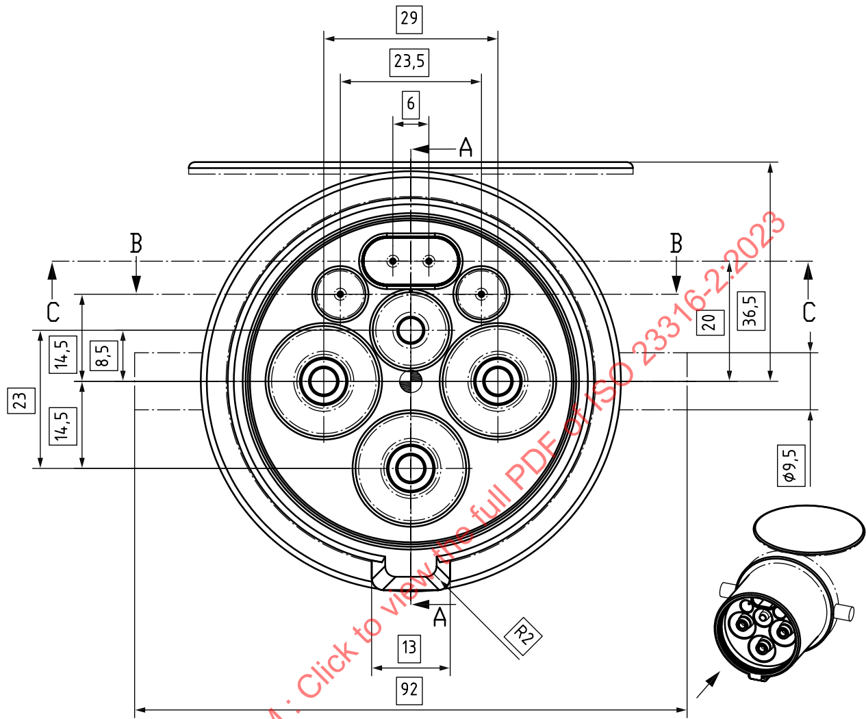
Figure 27 — Main front view of the implement side in minimum material model
