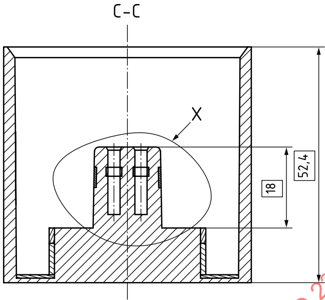
Figure 15 — Main front view, section C-C
