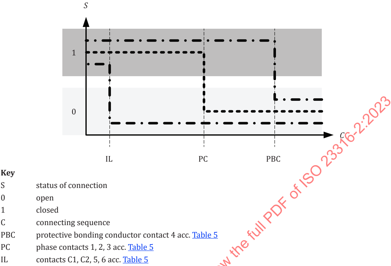
Figure 40 — Disconnecting sequences of contacts
