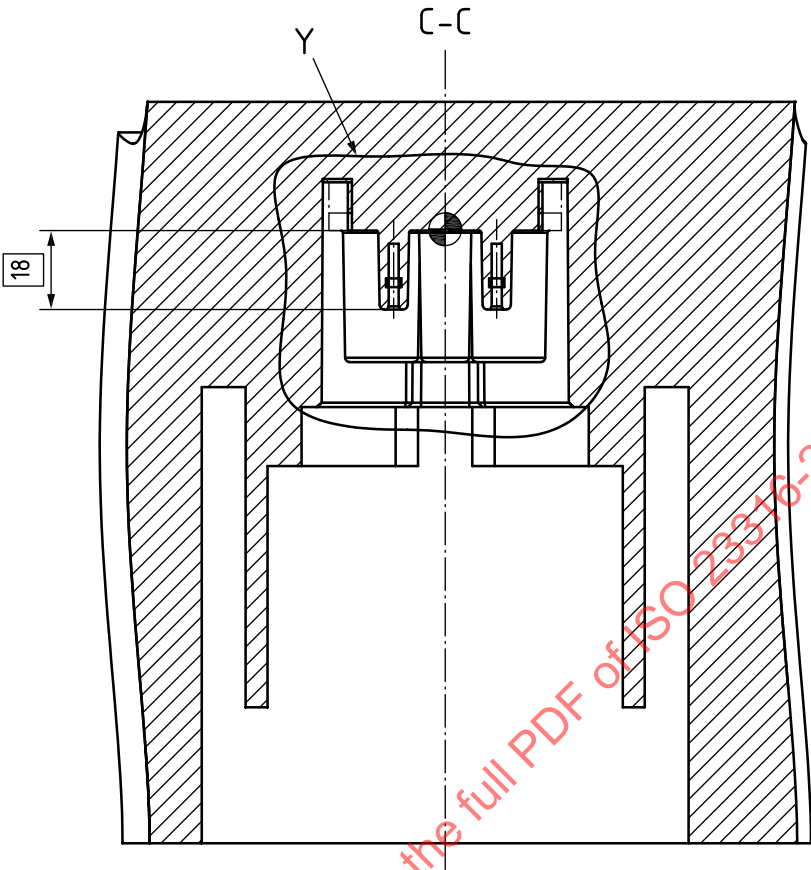
Figure 5 — Main front view, section C-C
