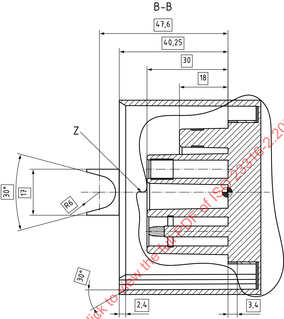
Figure 13 — Main front view, section B-B
