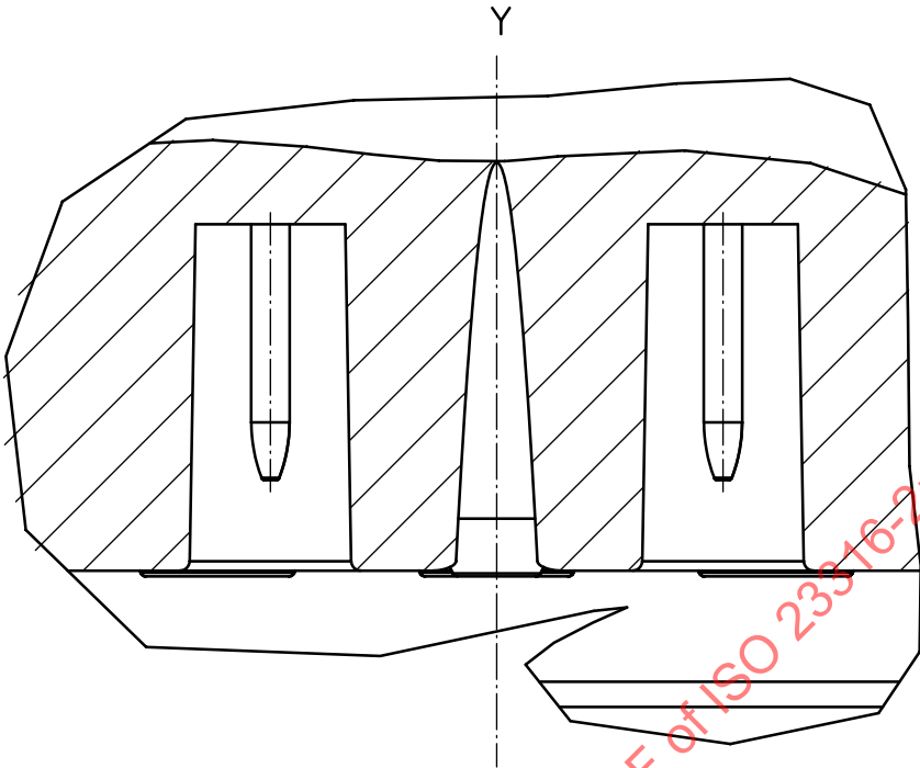
Figure 31 — Main front view, section B-B, detail Y
