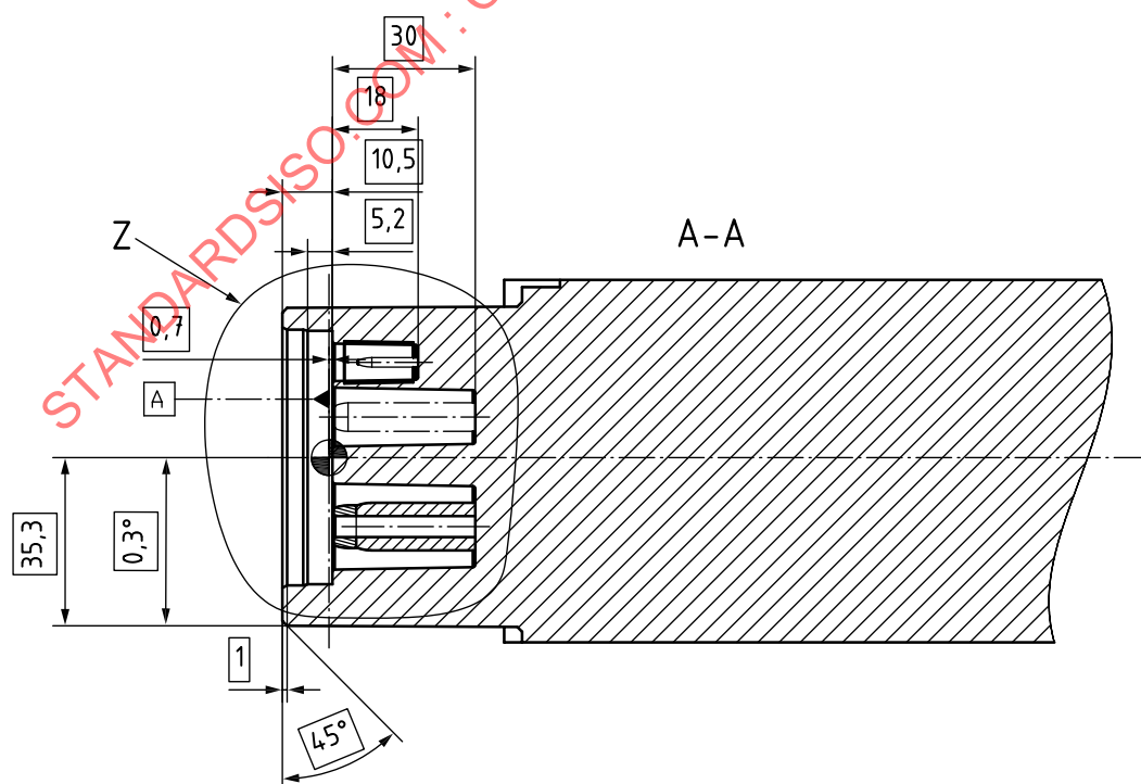
Figure 18 — Main front view, section A-A
