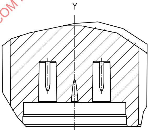
Figure 22 — Main front view, section B-B, detail Y
