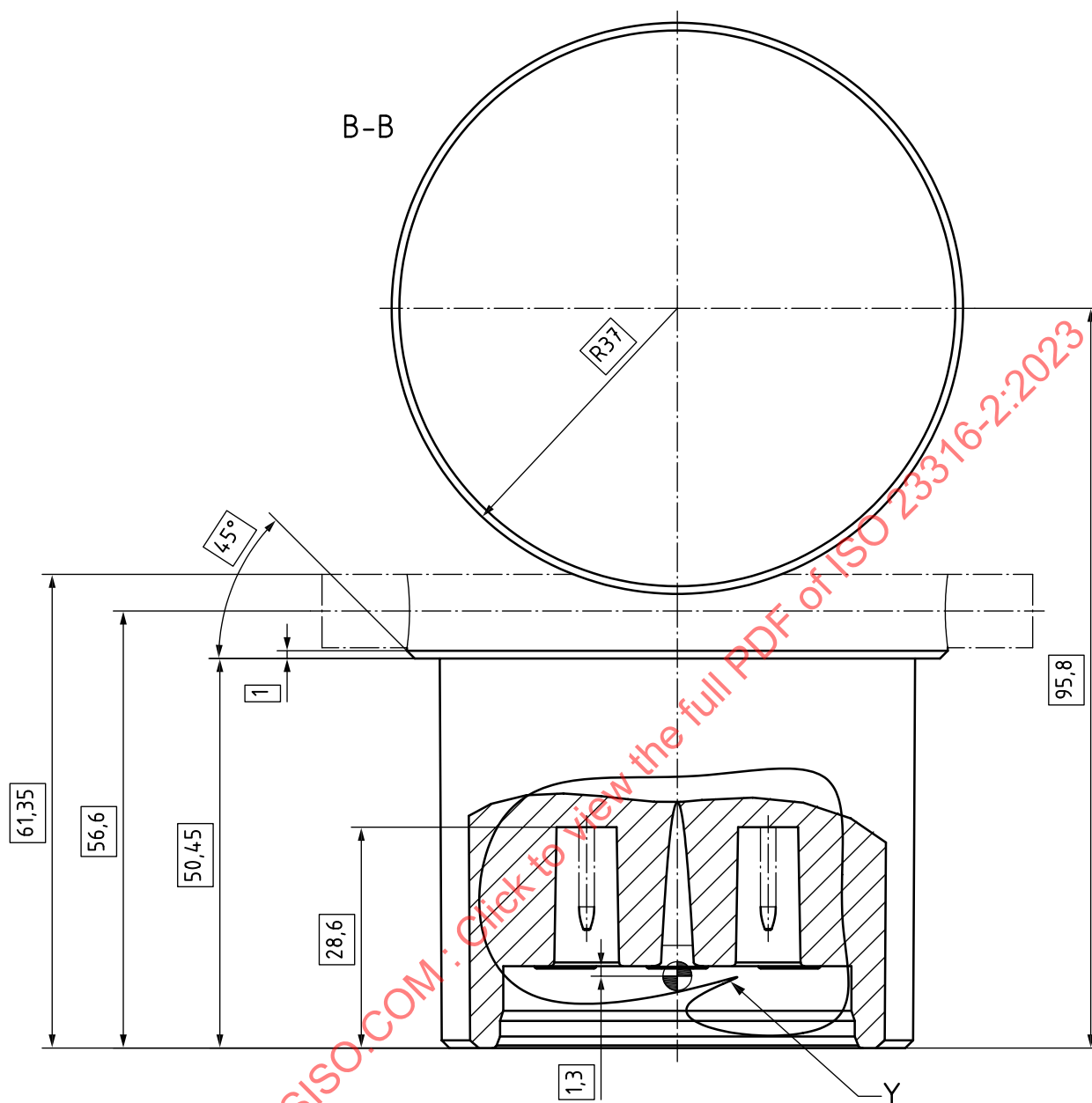
Figure 30 — Main front view, section B-B
