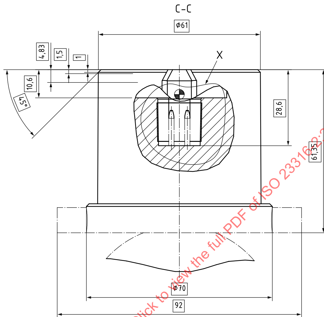
Figure 28 — Main front view, section C-C
