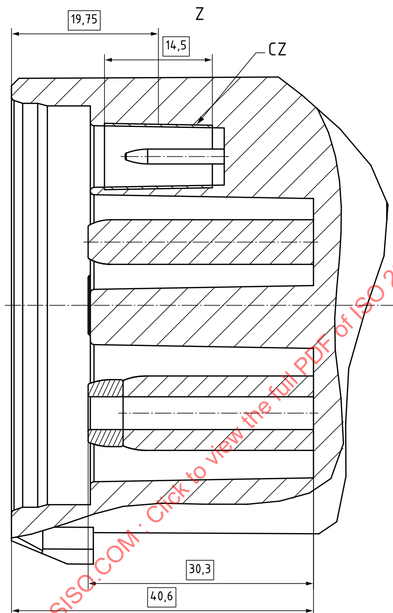
Figure 33 — Main front view, section A-A, detail Z
