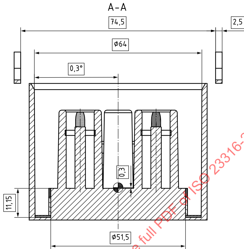
Figure 10 — Main front view, section A-A
