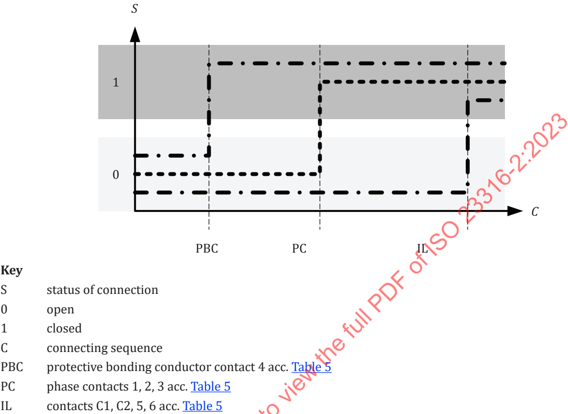
Figure 39 — Connecting sequences of contacts
