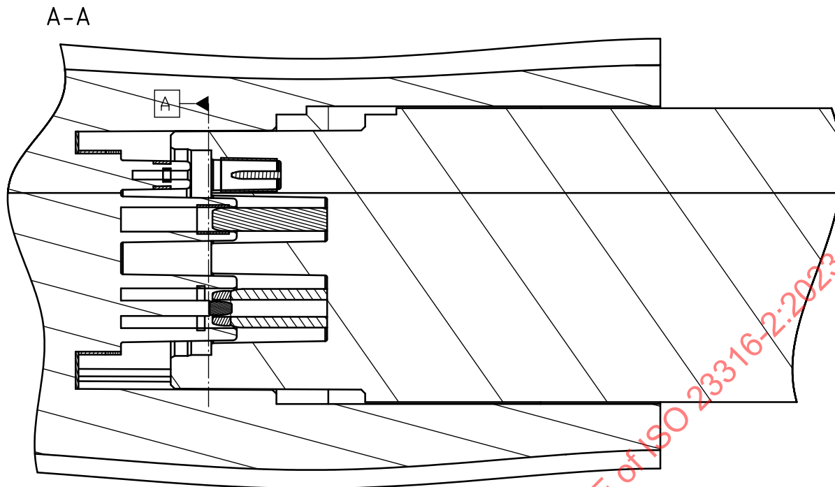
Figure 36 — Power pins connecting sequence
