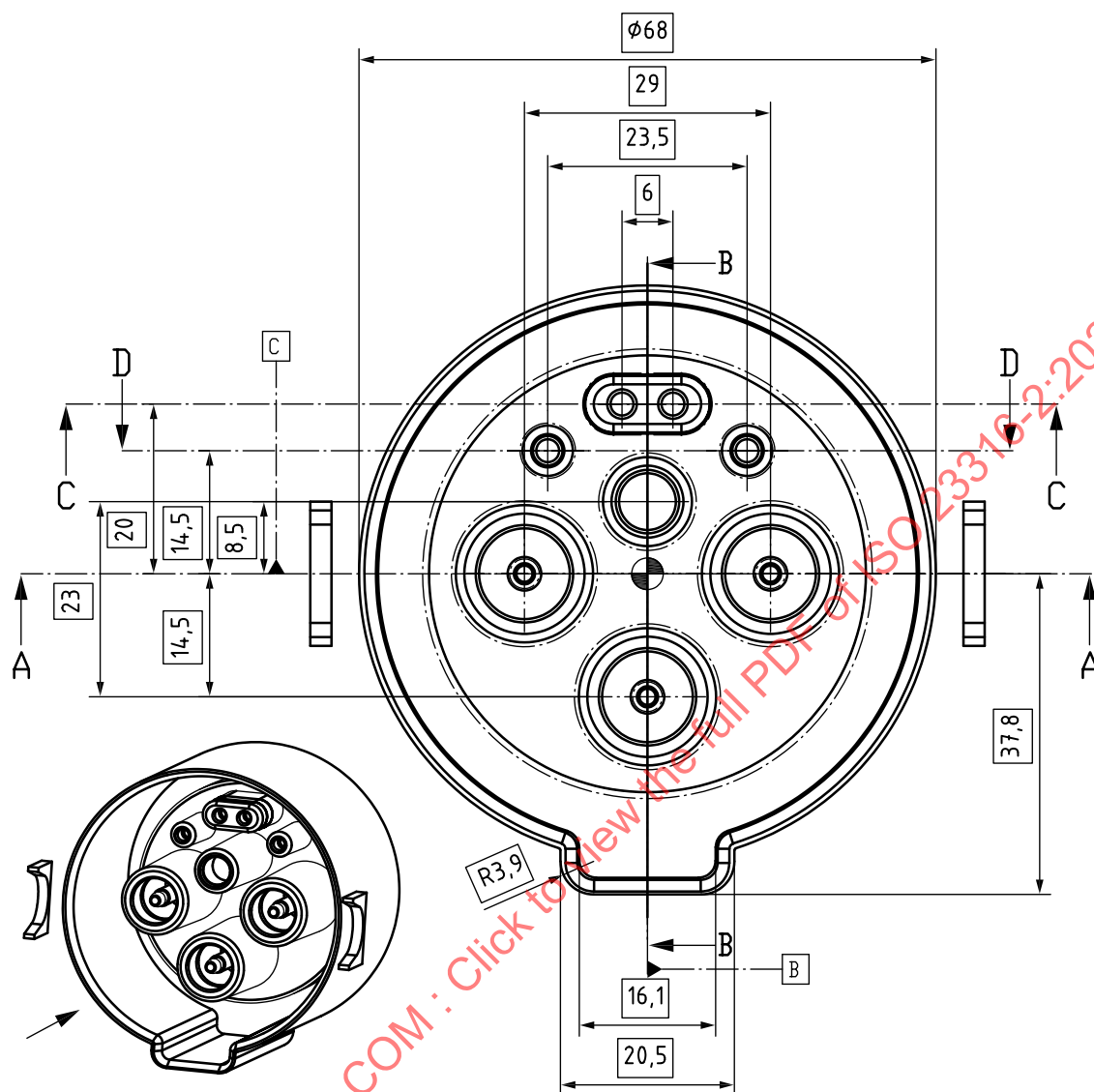
Figure 9 — Main front view of the tractor side in minimum material model
