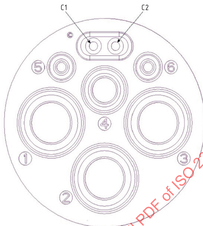
Figure 41 — Tractor side connector face view
