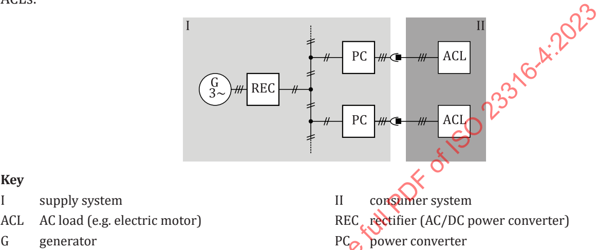
Figure 3 — Single consumer system schematic
