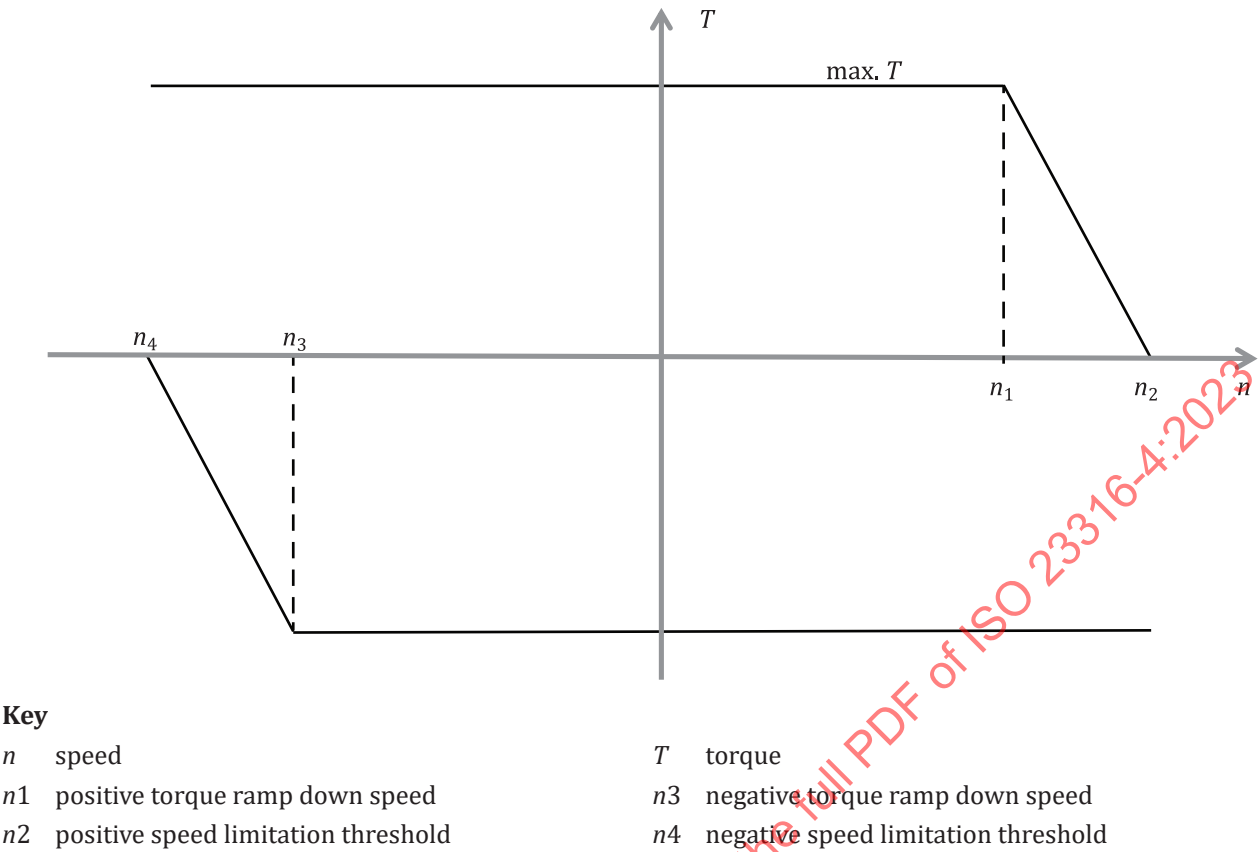
Figure 7 — Speed dependent torque derating
