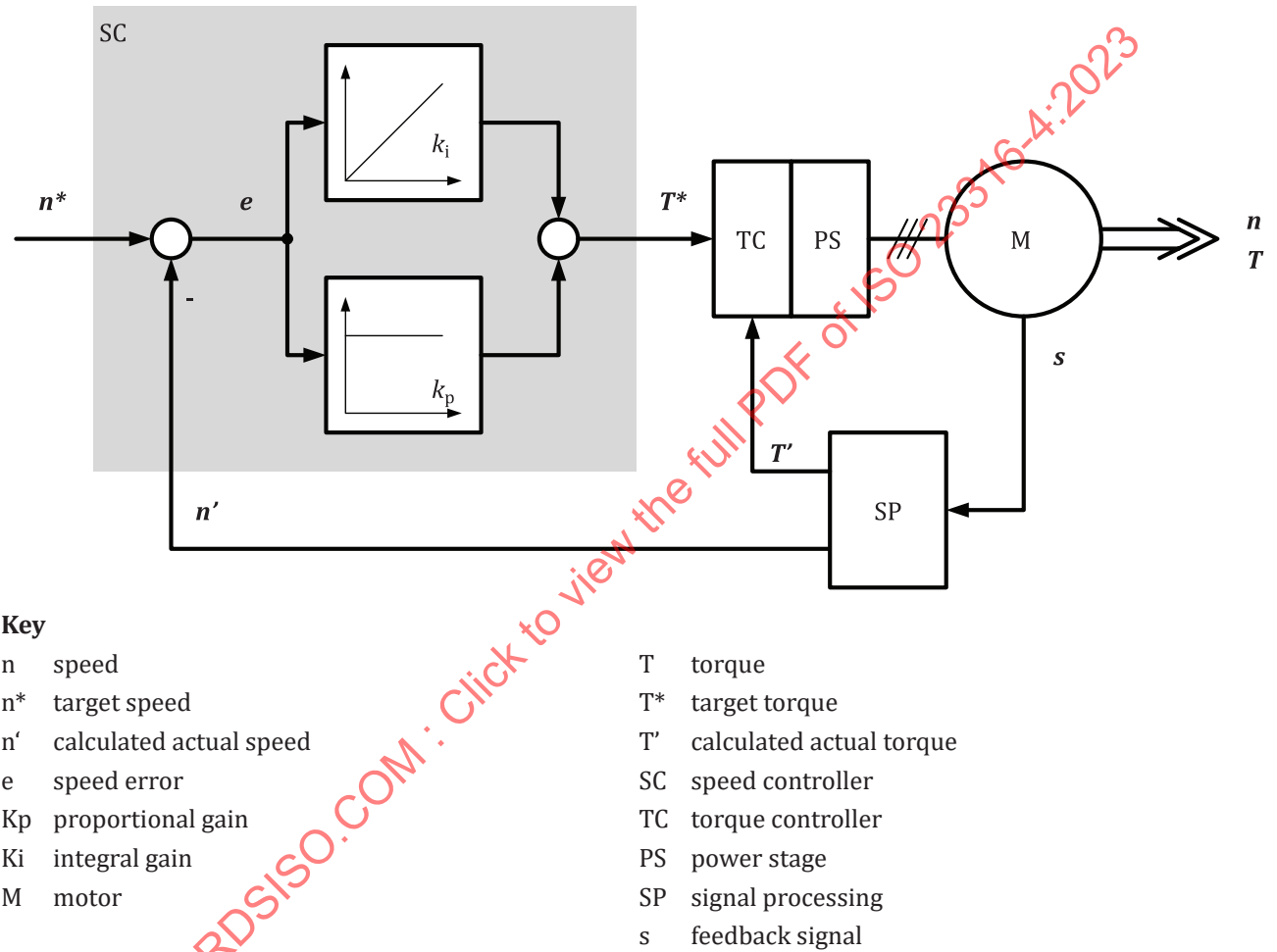
Figure 8 — Speed controller
