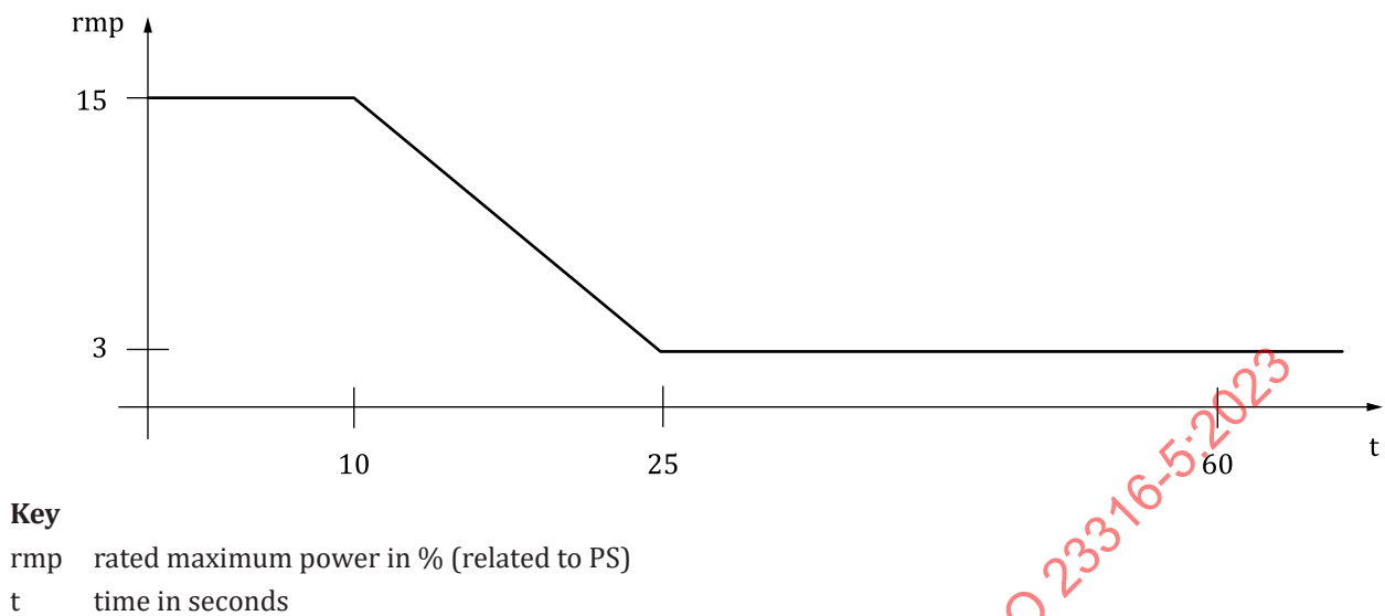
Figure 11 — Source energy feedback requirements
