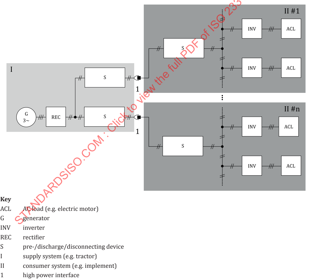
Figure 3 — Configuration with several parallel CS each at a separate connector
