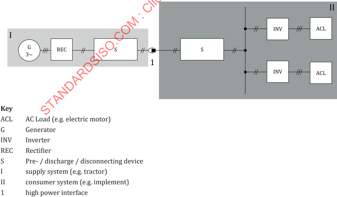
Figure 2 — Single implement block diagram
