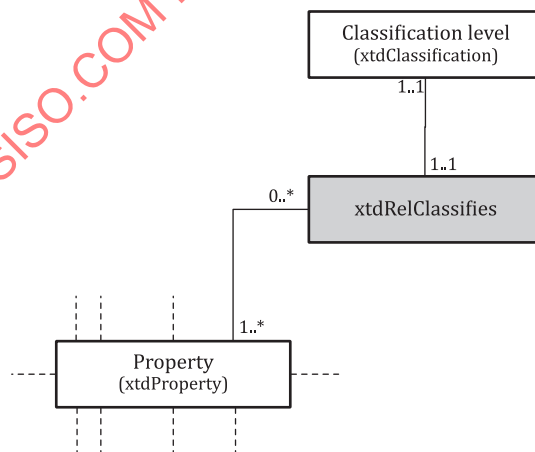
Figure 7 — Making a relationship between property and a classification level
