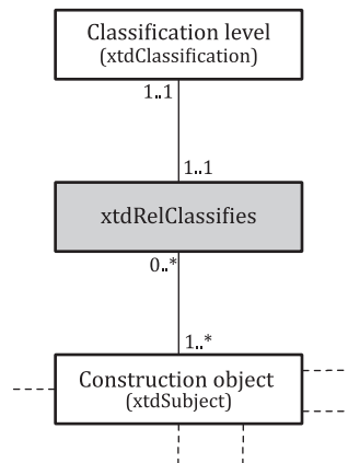
Figure 5 — Making a relationship between construction object and a classification level
