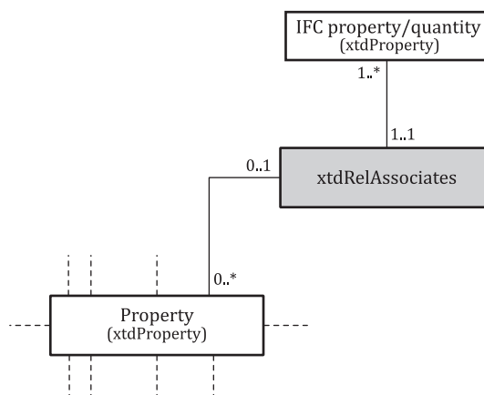
Figure 3 — Making a relationship between property and IFC property/quantity
