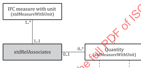
Figure 4 — Making a relationship between quantity and IFC measure with unit
