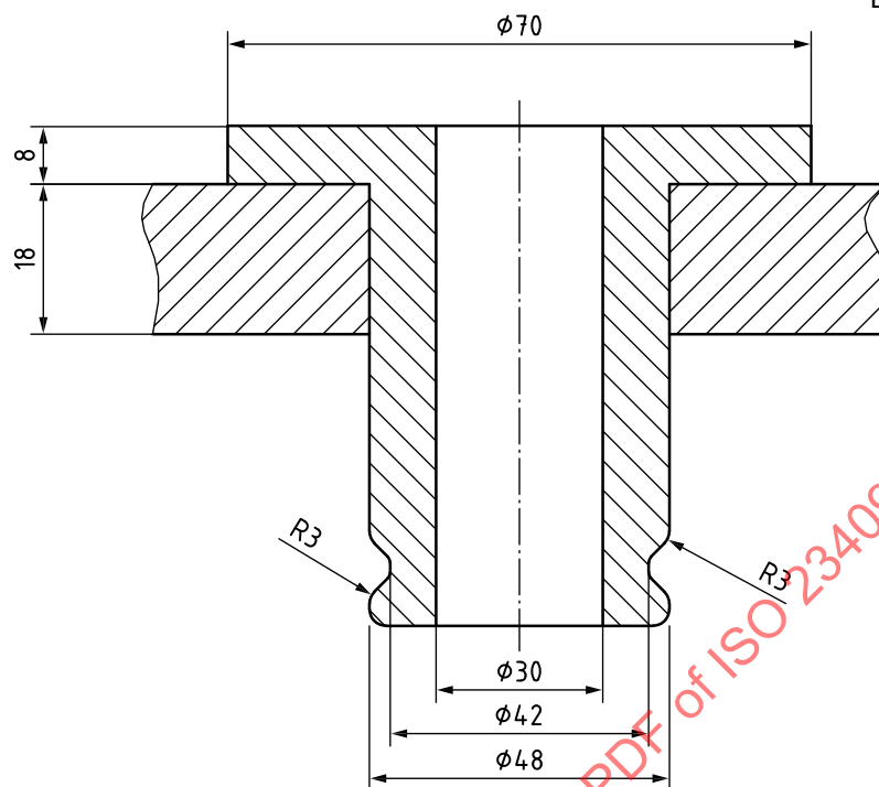
Figure J.3 — Examples of means of attaching the condom to the support
