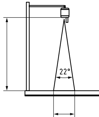
Figure 5 — Beam angle clearance
