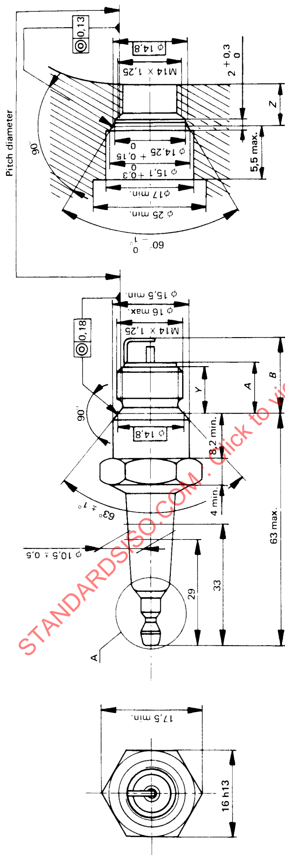
FIGURE 2 — Housing of the spark plug in the cylinder head
