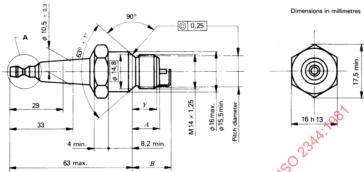
Figure 1 — Spark plug M 14 × 1,25 with conical seating
