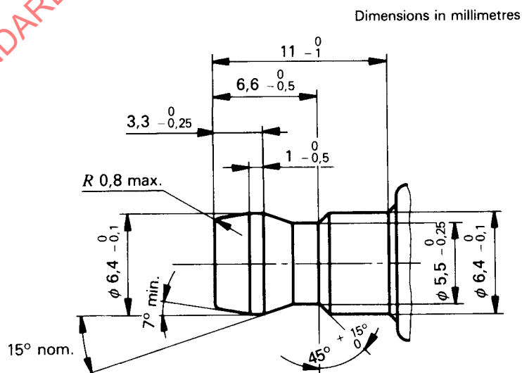
Figure 3 — Solid post terminal (detail A of figure 1)
