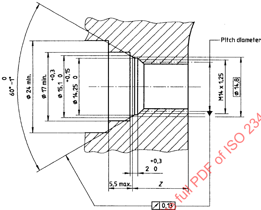
Figure 2 — Housing of spark-plug in cylinder head
