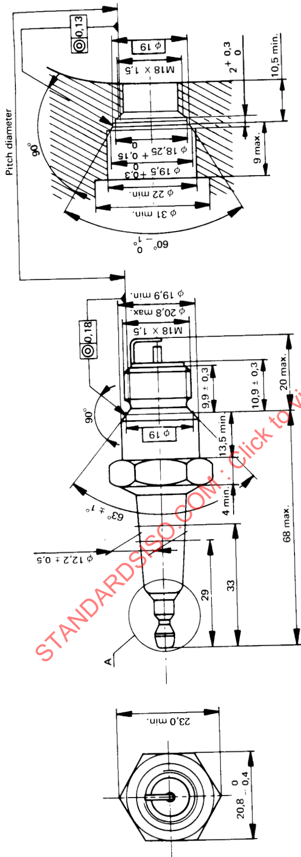
FIGURE 2 — Housing of the spark plug in the cylinder
