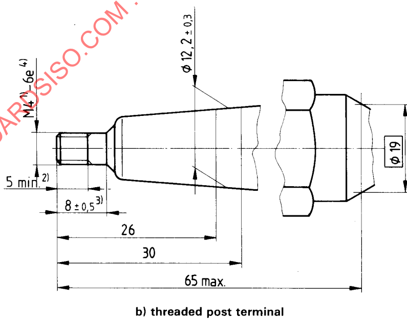
Figure 1 — M18 × 1,5 spark-plug with conical seating
