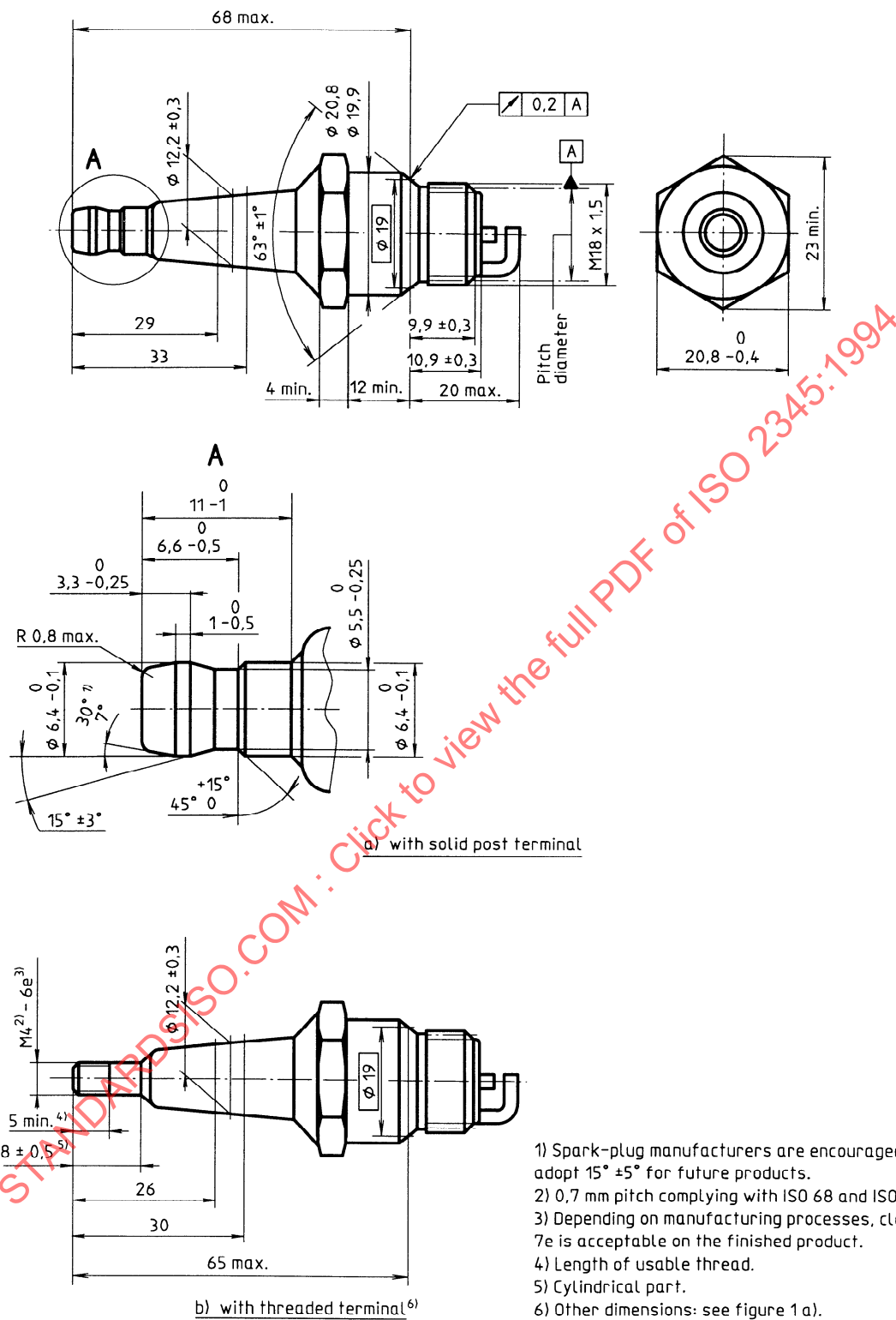
Figure 1 — M18 × 1,5 spark-plugs with conical seating
