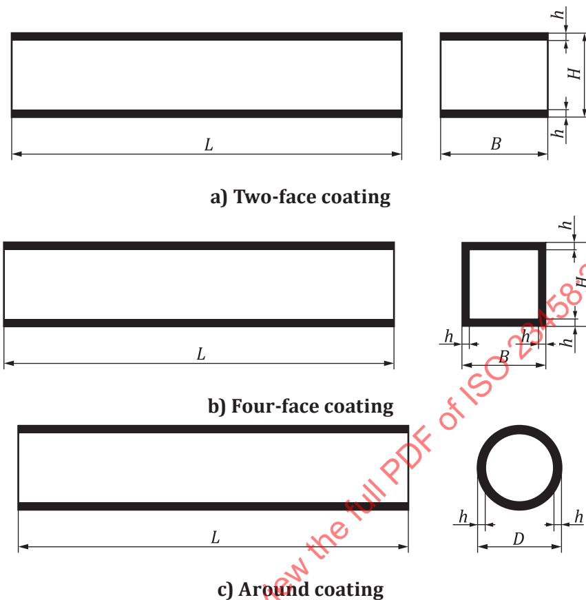
Figure 2 — Schematic of symmetrical structure of test pieces with different coating configurations for the thermal expansion coefficient tests
