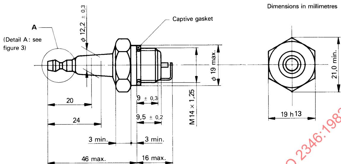
Figure 1 — Compact spark plug M 14 x 1,25 with flat seating
