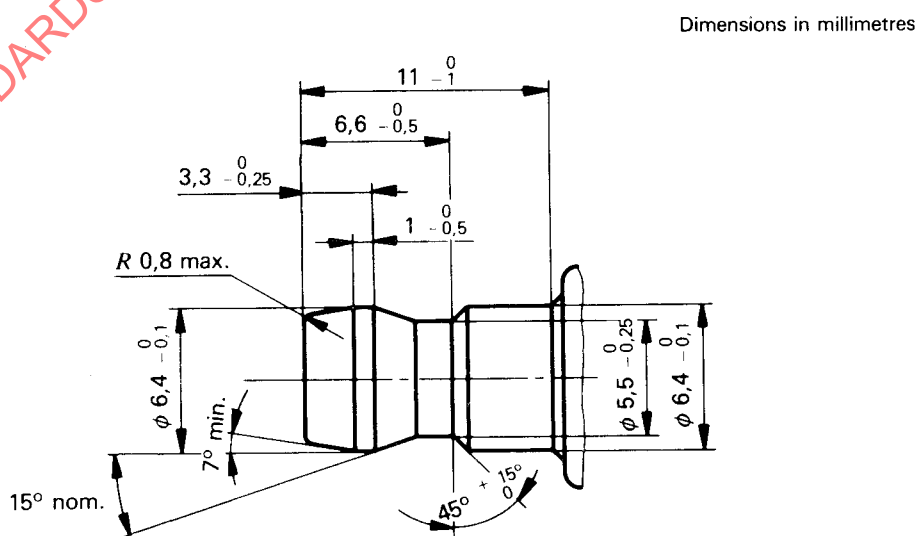
Figure 3 — Solid post terminal (detail A of figure 1)
