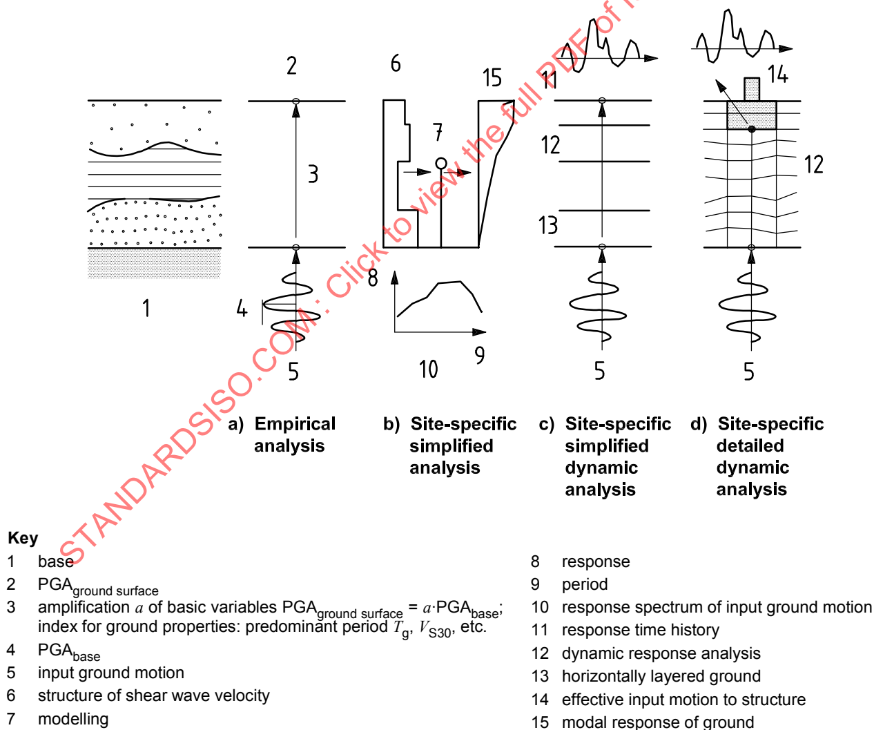
Figure E.7 — Schematic figure of methods for site response analysis
