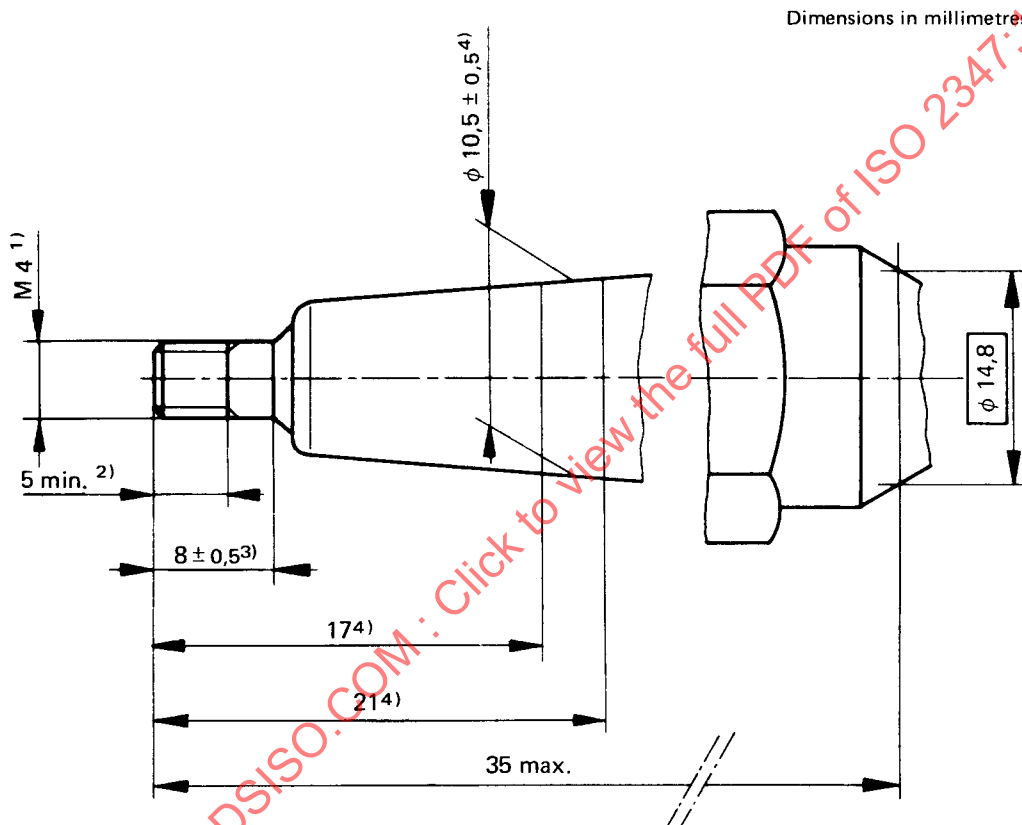
FIGURE 4 — Threaded terminal
