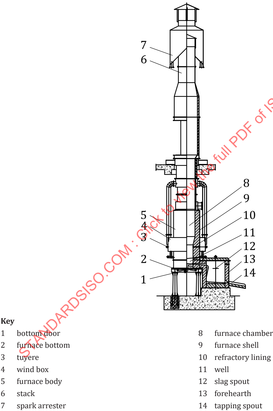
Figure A.1 — Example of cupola furnace structure
