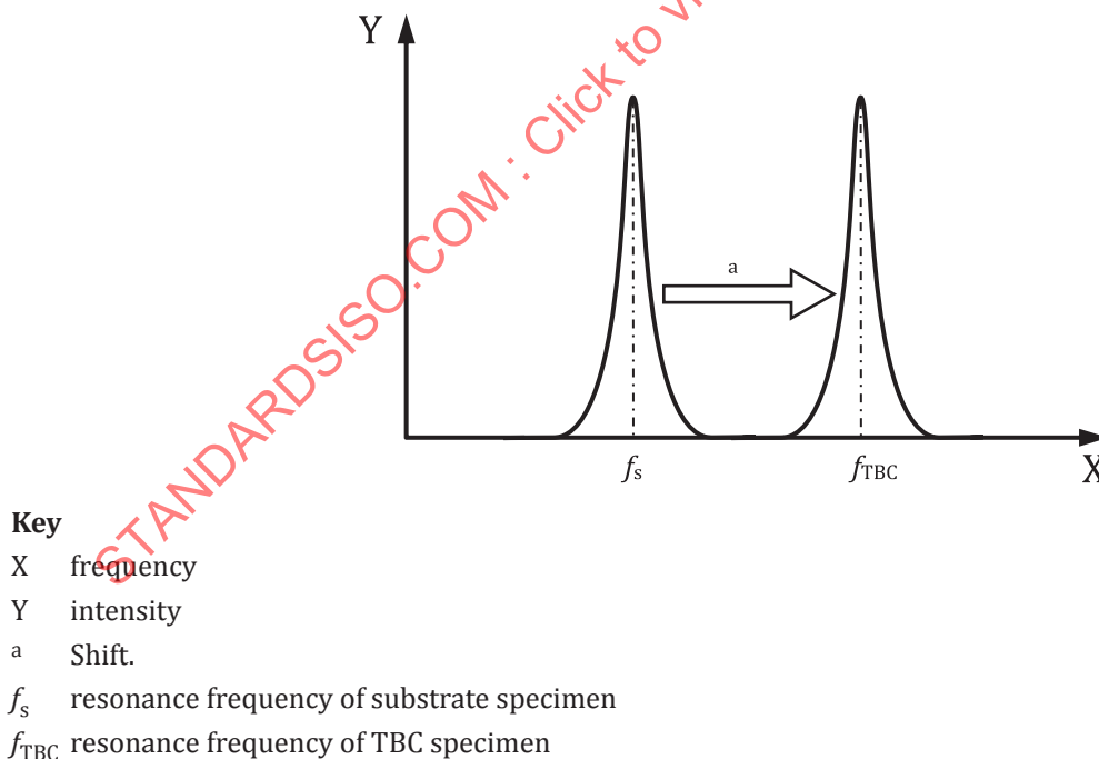
Figure 4 — Schematic illustration of the resonance frequencies of substrate and TBC specimens
