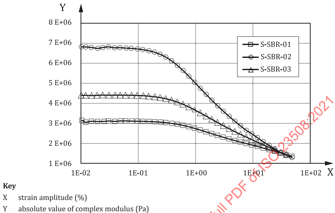
Figure C.1 — Results of the strain dependency
