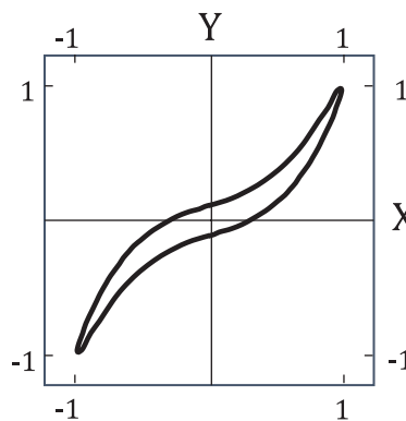
Figure B.1 — Example of an elliptical Lissajous figure
