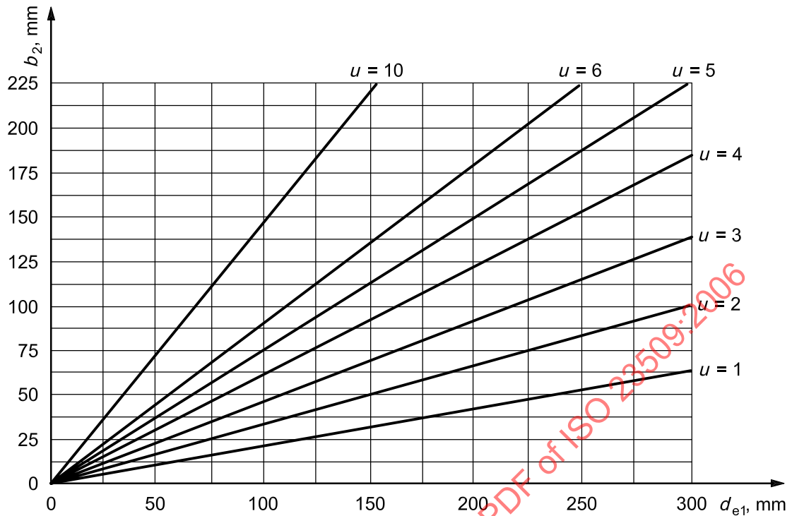
Figure B.6 — Face width of spiral bevel gears operating at 90° shaft angle
