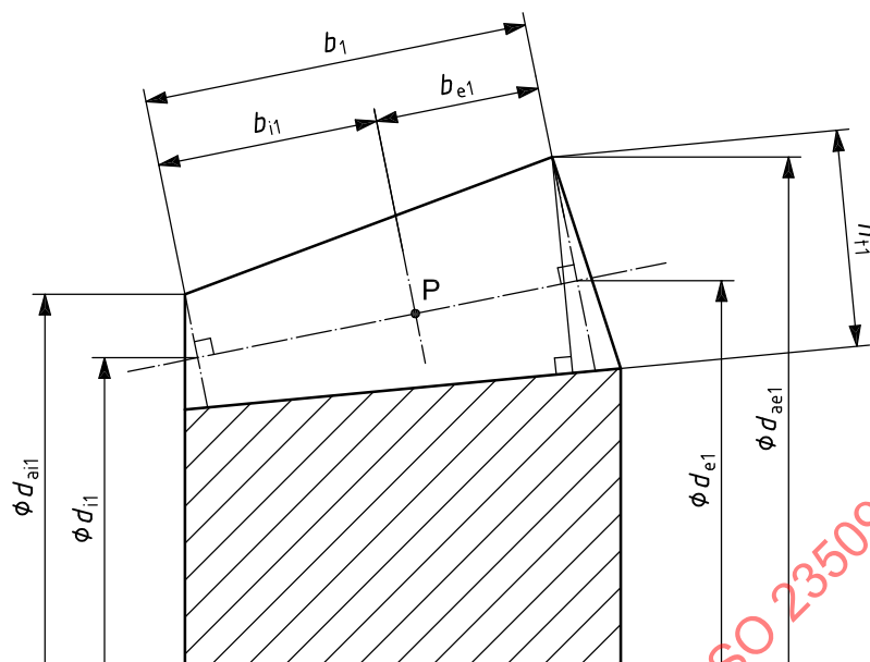
Figure A.3 — Pinion face width and inner and outer diameter
