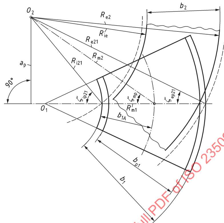
Figure A.4 — Determination of pinion spiral angle in pitch plane
