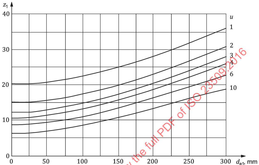
Figure B.4 — Approximate number of pinion teeth for spiral bevel and hypoid gears
