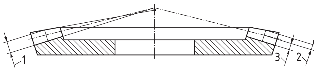
a) Standard depth taper
