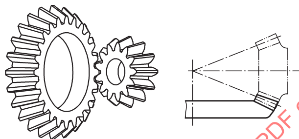
Figure 4 — Straight bevel
