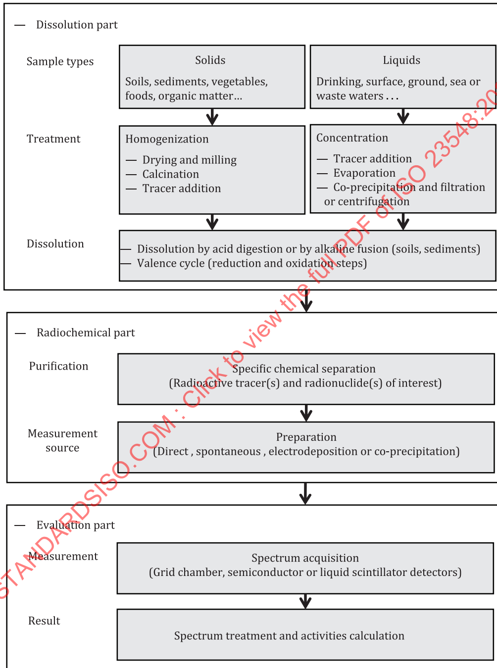
Figure A.1 — Schematic diagram of generic alpha test method processes
