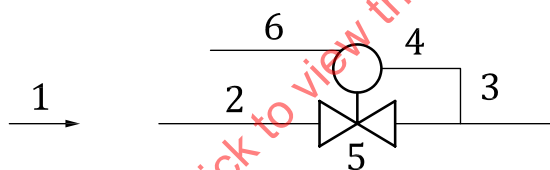
Figure I.1 — Pressure reducing regulator (constant pressure control)
