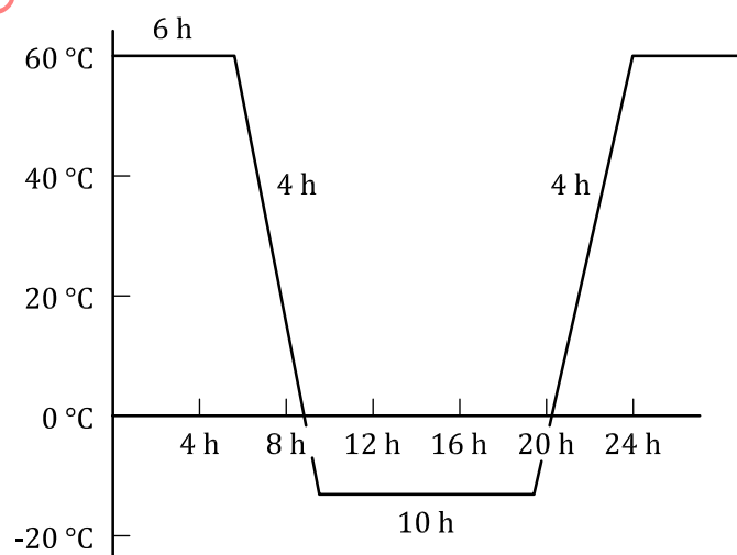
Figure J.6 — Temperature cyclic test
