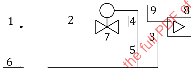
Figure I.5 — Flow rate regulator (staged flow rate control / preheated air)
