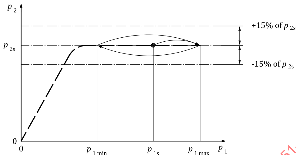
Figure J.4 — Graph of performance Class D regulator
