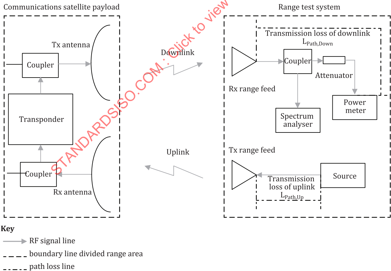
Figure A.1 — EIRP test schematic diagram of full link wireless transmission route
