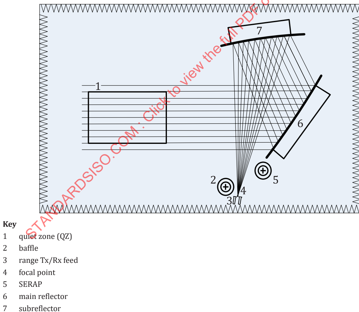
Figure 3 — Schematic of baffle and SERAP's position
