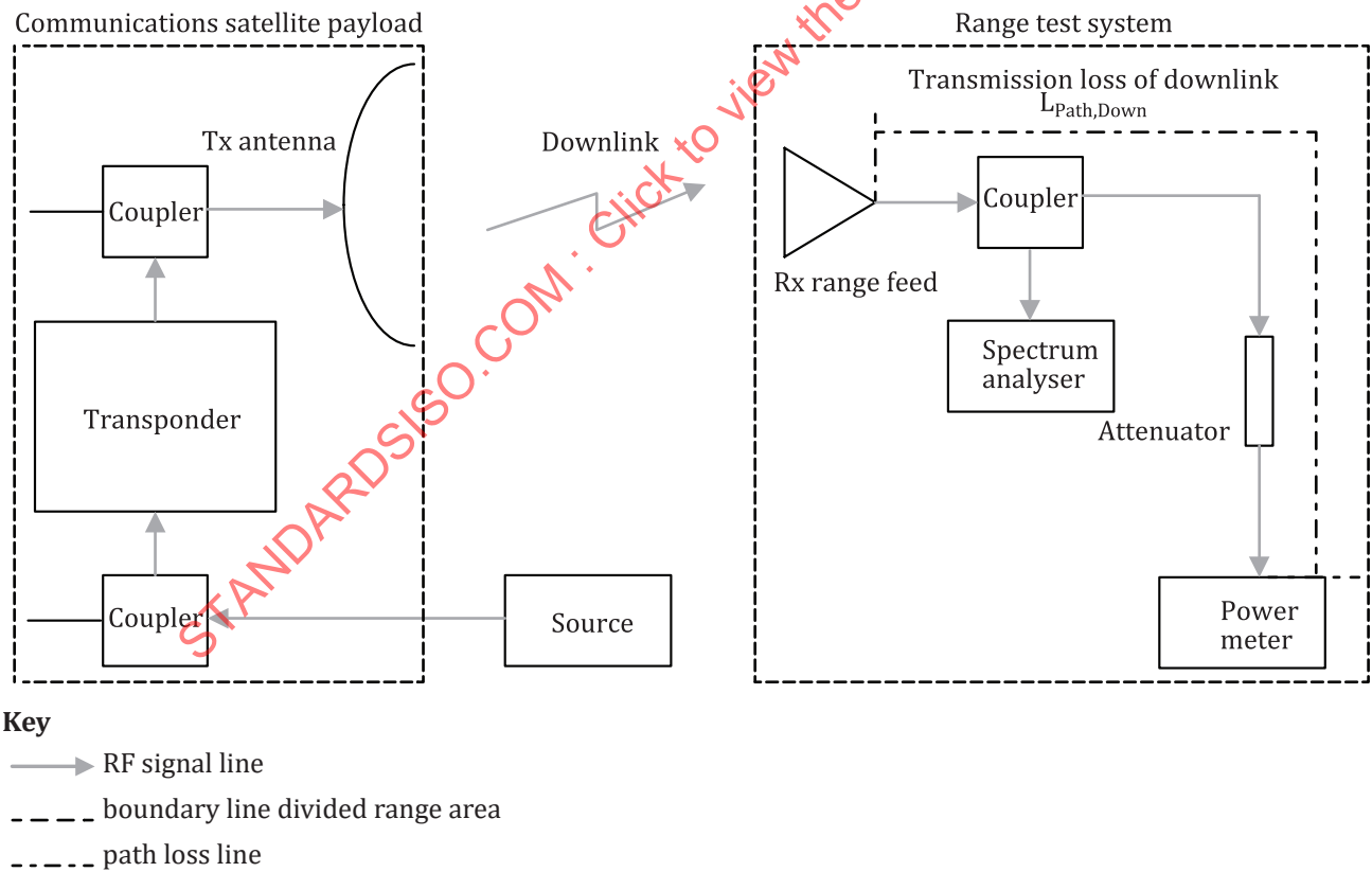
Figure A.2 — EIRP test schematic diagram of downlink wireless transmission route
