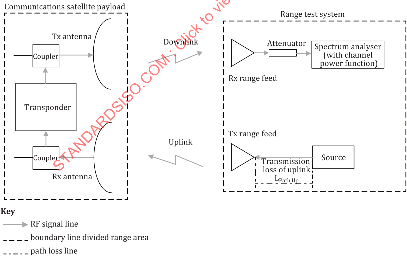
Figure B.1 — G/T -test schematic diagram of full link wireless transmission route in fixed gain mode
