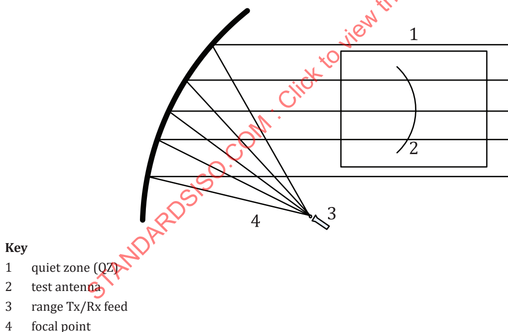
Figure 1 — Schematic representation of a compact range using a reflector and feed
