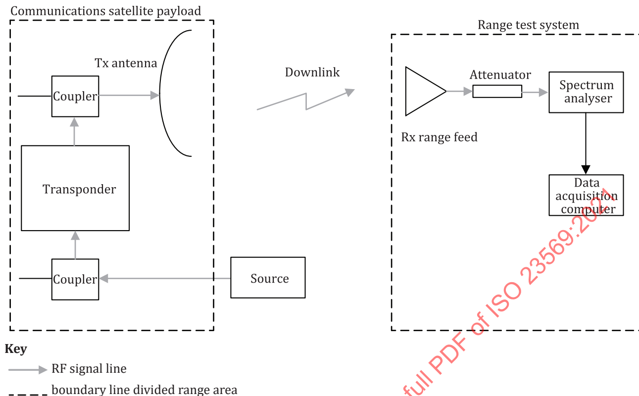
Figure D.3 — Output AFR test schematic diagram of downlink wireless setup
