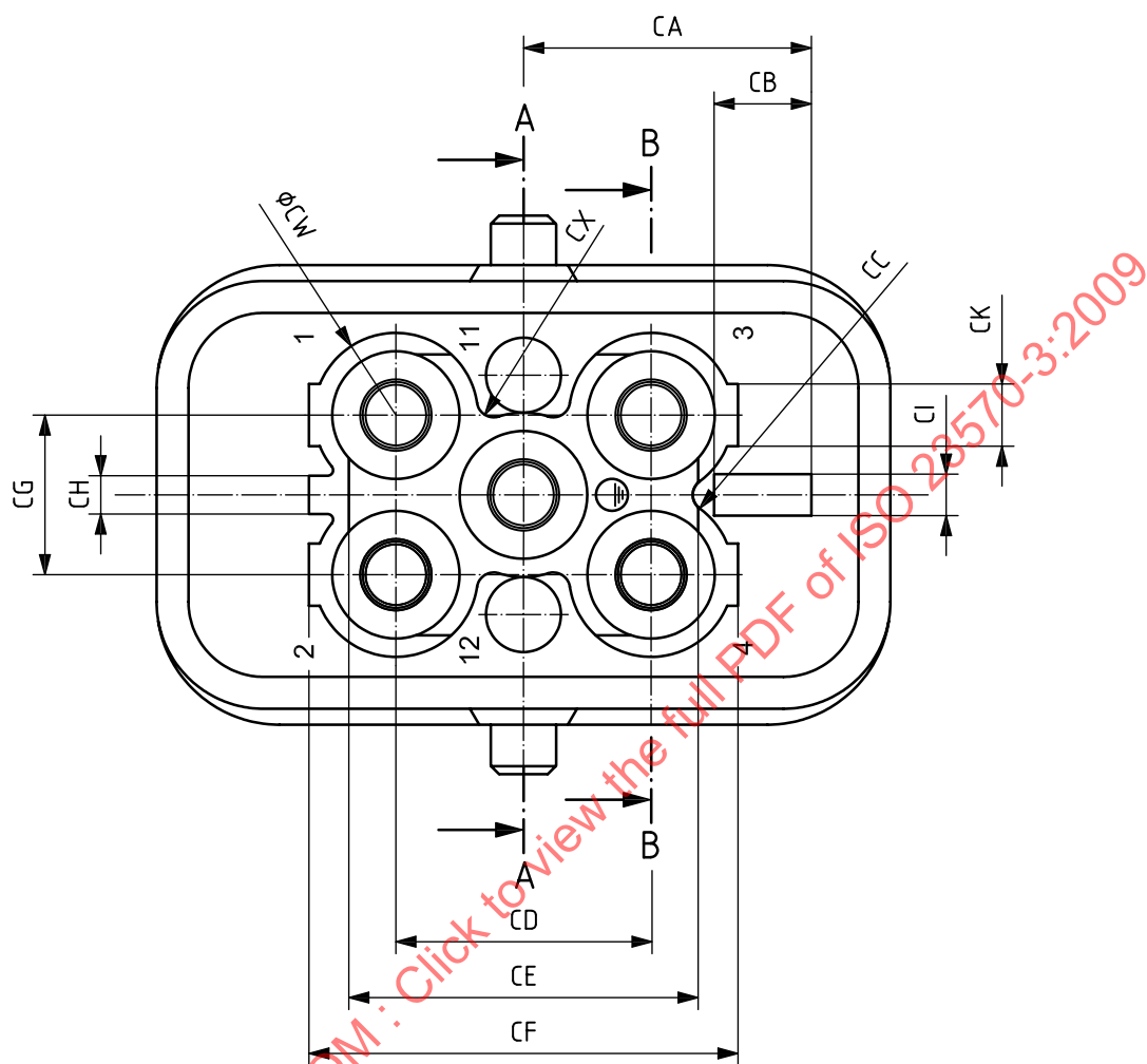
Figure A.4 — Female power bus connector
