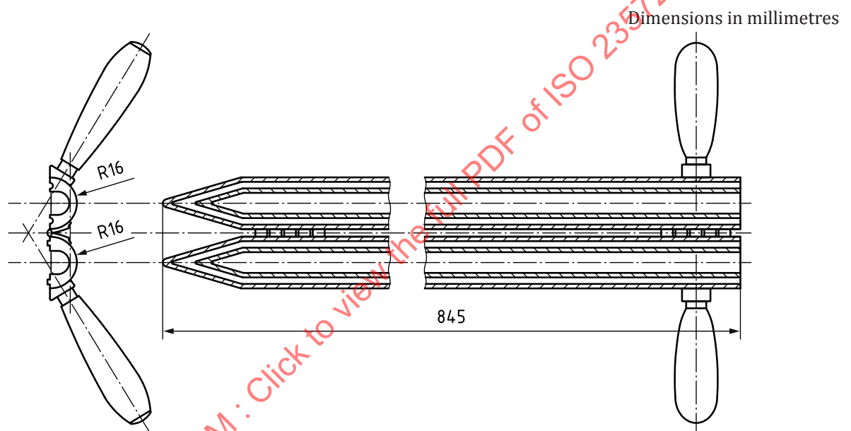
Figure 3 — Allen Auerbach auger
