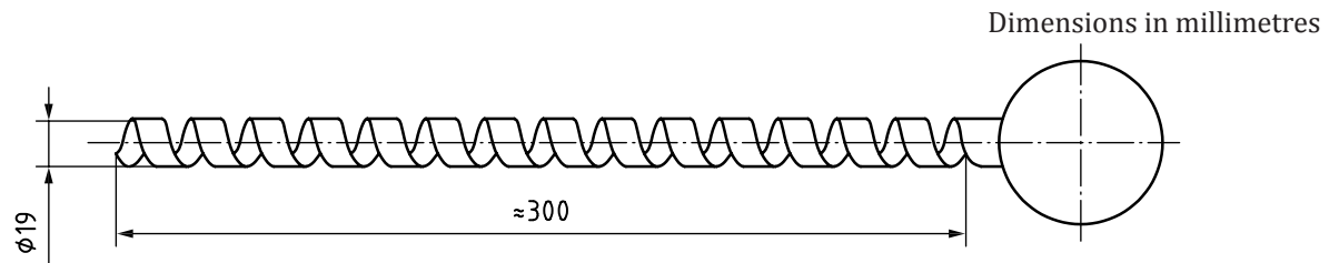
Figure 2 — Ship auger
