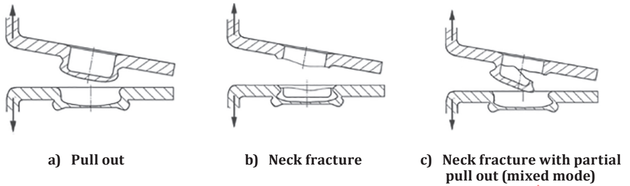
Figure A.3 — Typical failure modes of clinch joints
