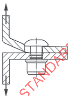
a) Sheet material pull out
