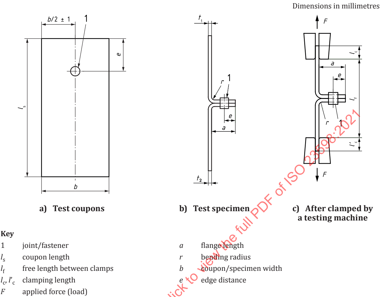
Figure 1 — Test coupons, test specimens and the clamping state for mechanized peel testing
