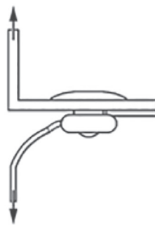
b) Closed head pull out in lower sheet
