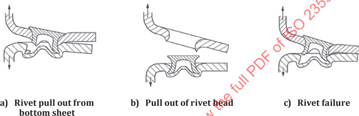
Figure A.1 — Typical failure modes of semi-tubular self-piecing rivet joints
