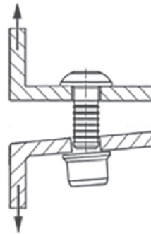
b) Bolt collar failure
