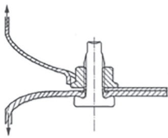
a) Pull out of weaker sheet material
