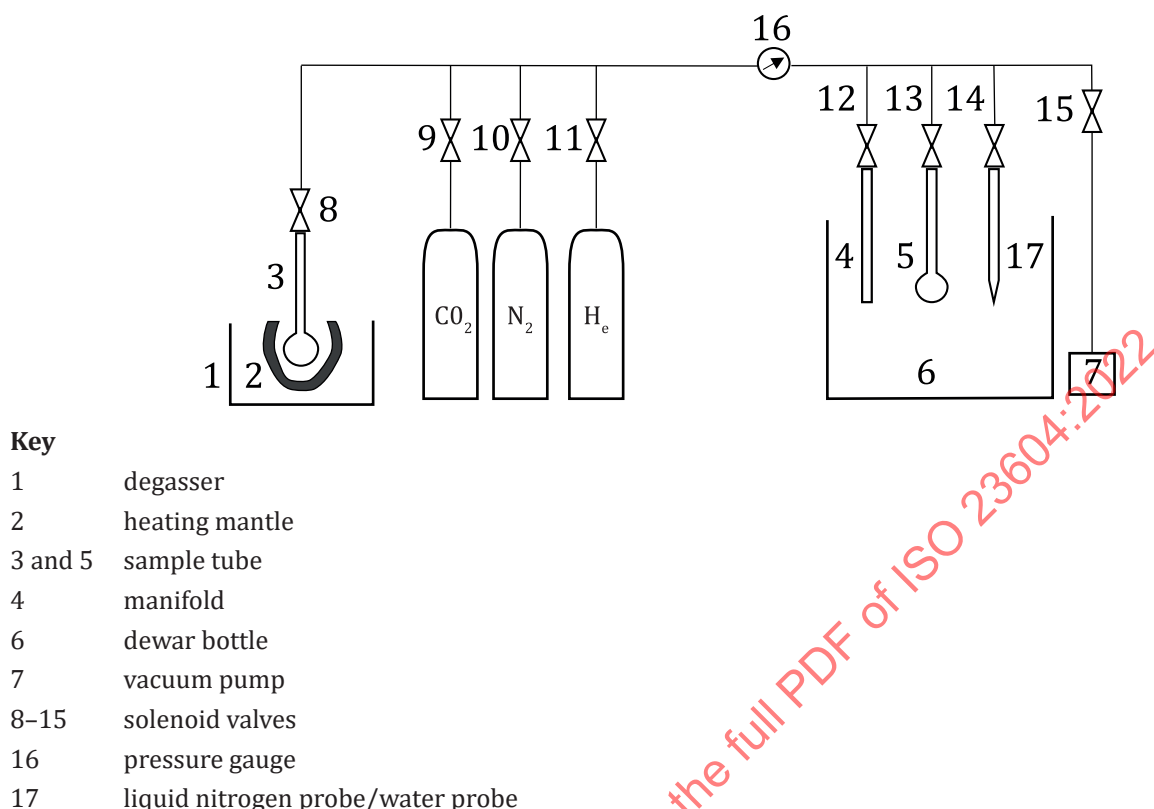
Figure 1 — Specific surface area analyser
