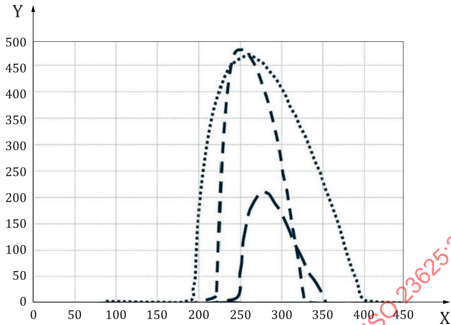
a) Accelerating rate calorimetry (ARC) of 18650 cells with different positive active materials (cathode)
