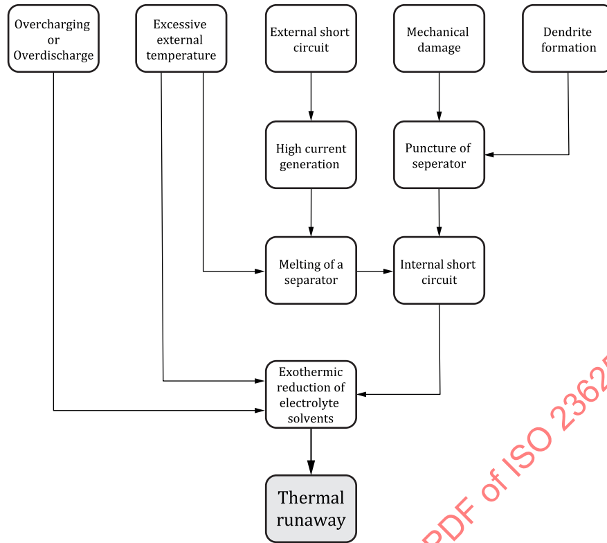
Figure A.1 — Causes of thermal runaway
