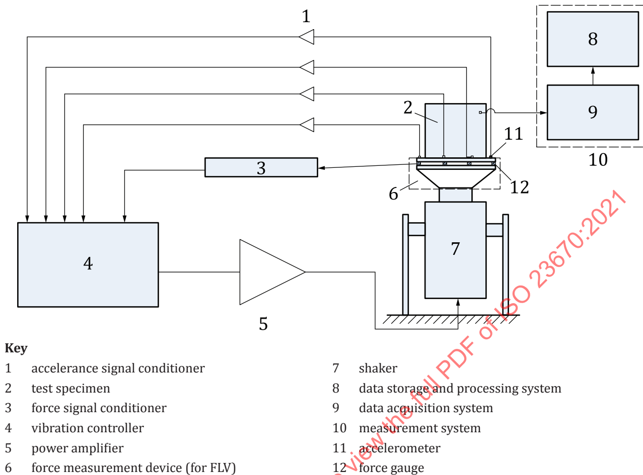
Figure 1 — Illustration of a force limited testing system
