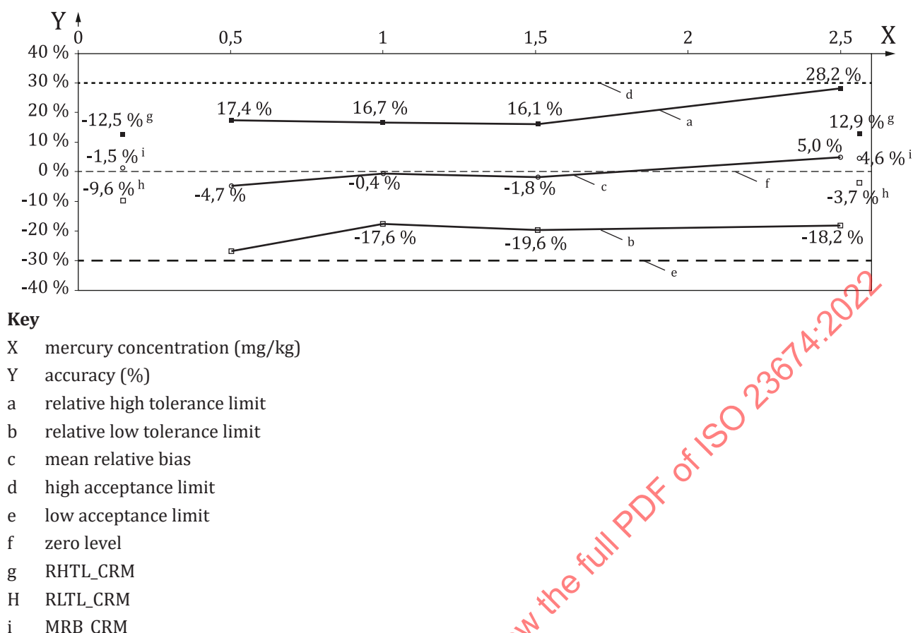
Figure A.2 — Accuracy profile for mercury validating this document in the range 0,5 mg/kg to 2,5 mg/kg (ppm)
