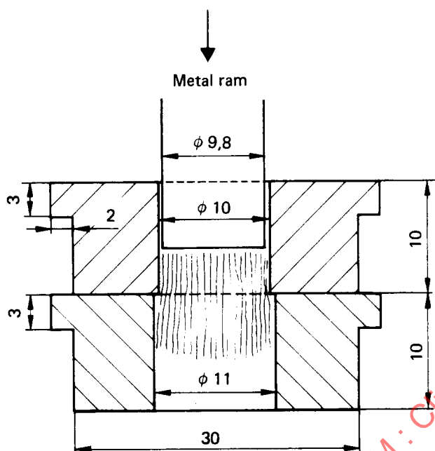
FIGURE 3 — Transferring the wad of fibres
