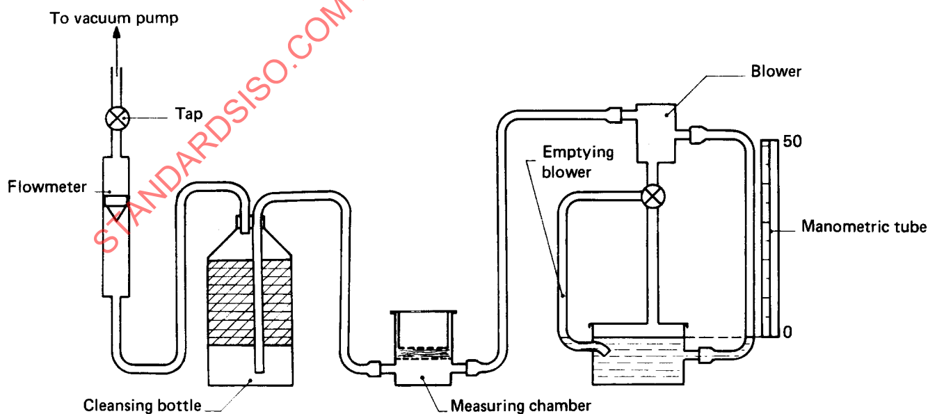
FIGURE 4 — Test apparatus
