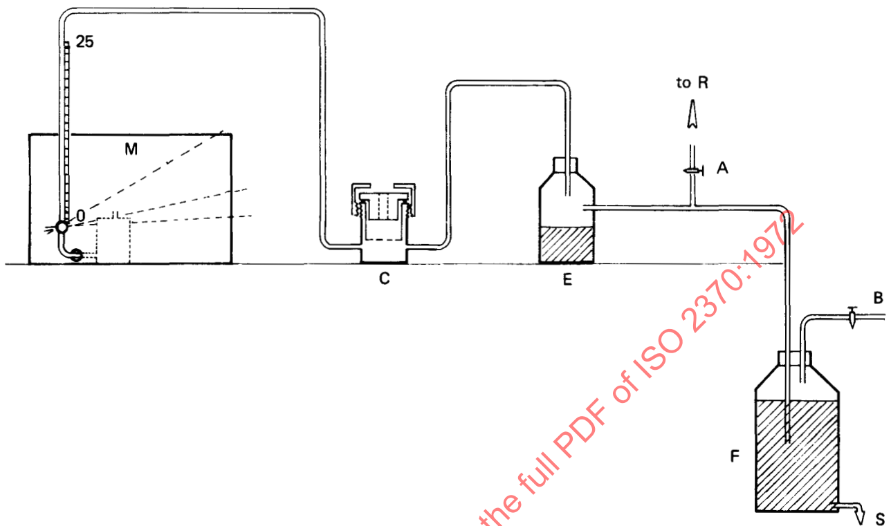
FIGURE 1 — Test apparatus
