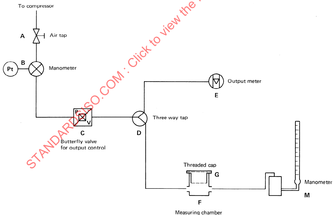
Figure 1 — Apparatus for the reference method
