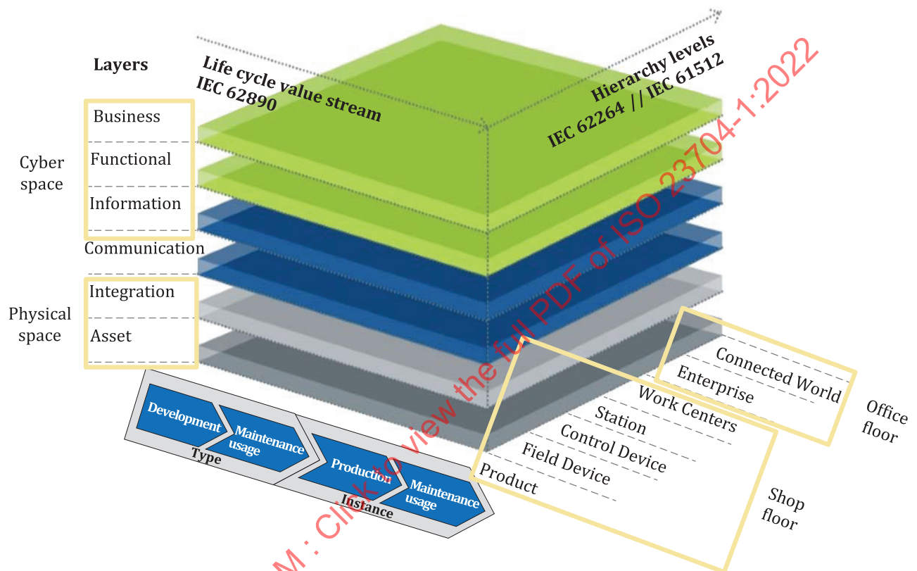
Figure A.1 — Analogy of RAMI 4.0 from the cyber-physical perspective (based on IEC PAS 63088:2017, Figure 8, modified by the addition of yellow boxes)
