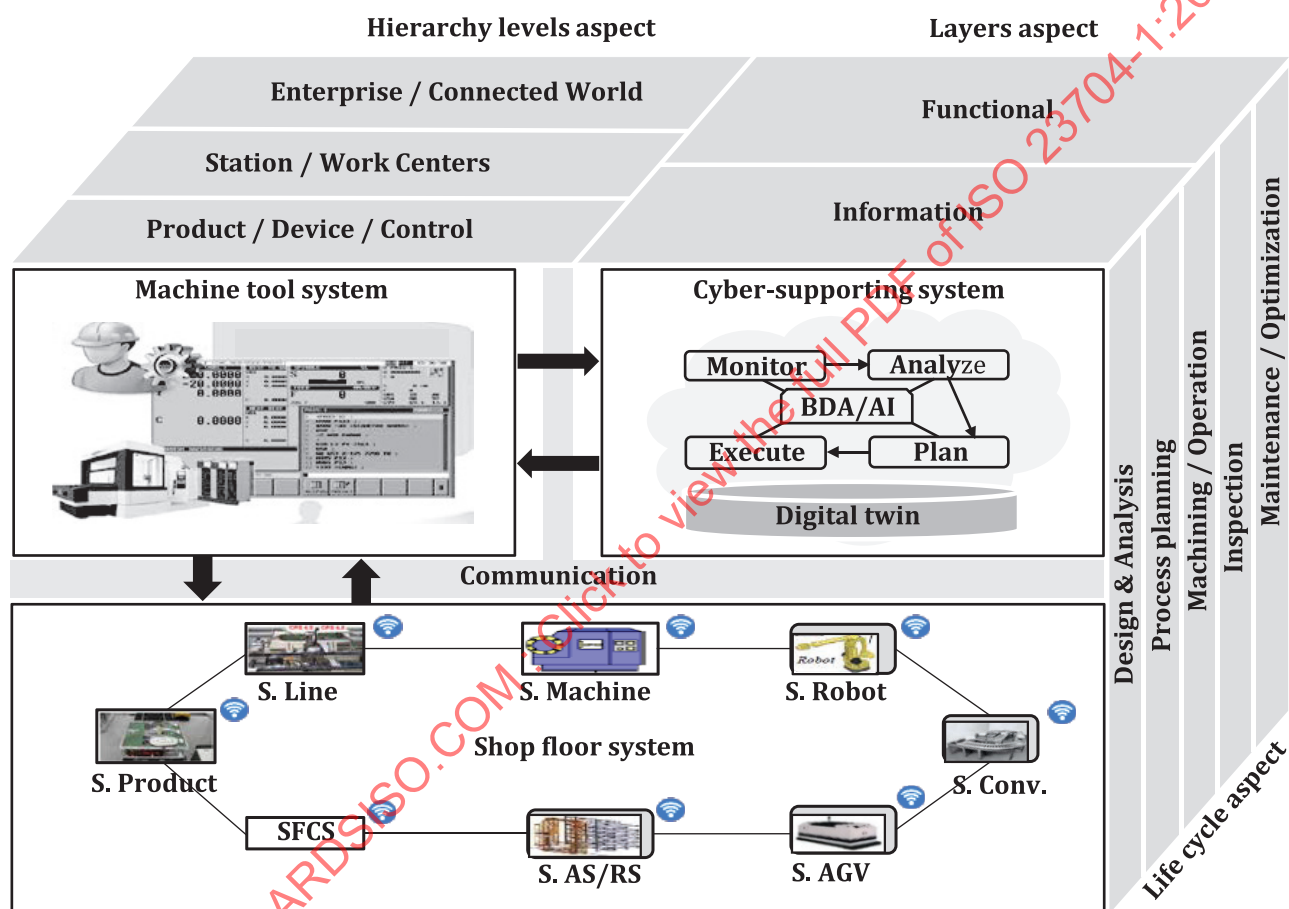
Figure A.3 — Concept of cyber-physically controlled smart machine tool systems (CPSMT)
