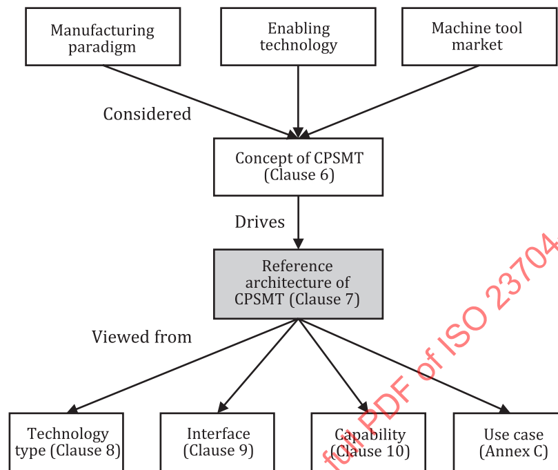
Figure 2 — Context of a CPSMT reference architecture
