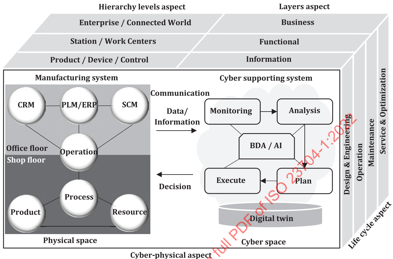
Figure A.2 — Cyber-physical manufacturing system (CPMS)
