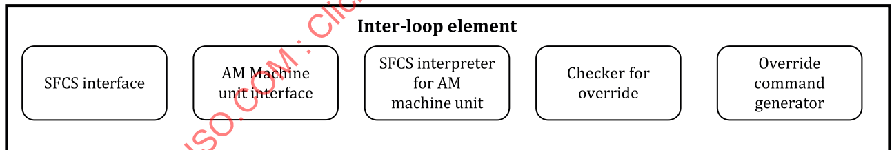
Figure 6 — Functional structure of the inter-loop element
