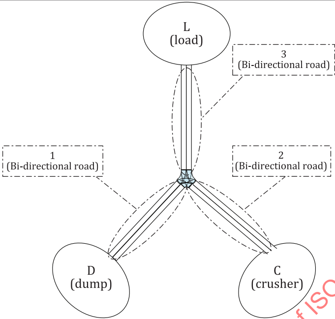
Figure 4 — Example of road level modelling
