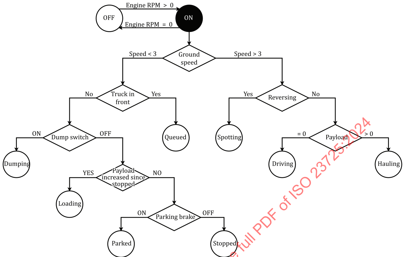
Figure 7 — Haul truck cycle
