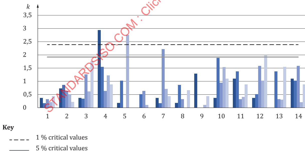
Figure A.2 — Mandel's intralaboratory consistency statistic, k , grouped by laboratories
