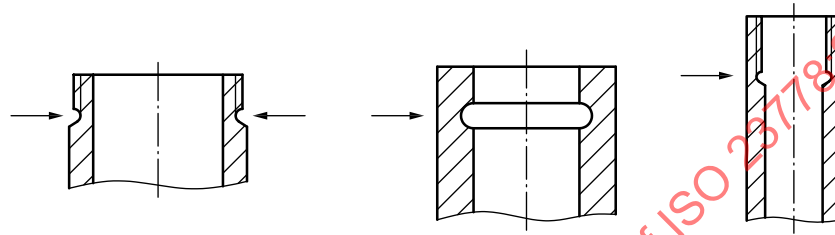
Figure 14 — Undercuts at thread run out
