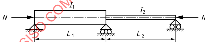
Figure A.6 — Buckling case E (two coupled Euler 2 cases)
