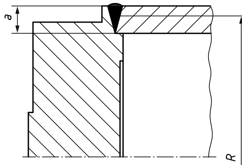
Figure 13 — Bottom weld
