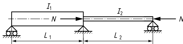
Figure A.7 — Buckling case F (Euler 2 case coupled with a rotational spring)
