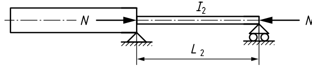
Figure A.4 — Buckling case C (regular Euler 2 case)
