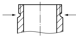
Figure 22 — Undercut for tube thread
