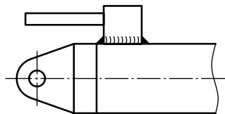
Figure 20 — Oil connector on piston side
