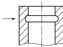
Figure 23 — Locking wire groove
