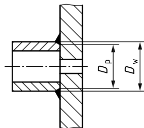
Figure 15 — Welded oil connector
