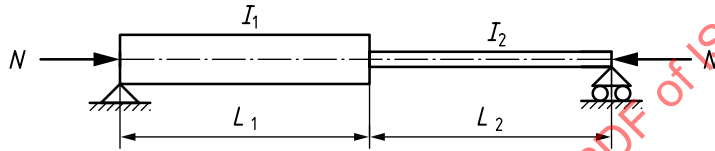
Figure A.5 — Buckling case D (as Euler 2 case, but with two different cross-sections)
