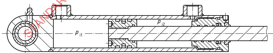
Figure 7 — Pushing cylinder, flange mounted with unsupported bottom
