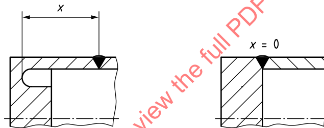
Figure 19 — Bottom weld
