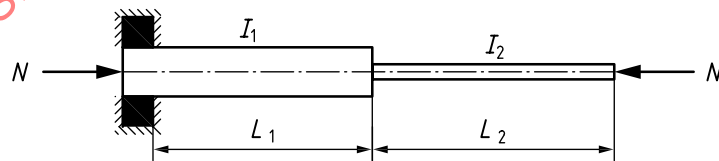
Figure A.3 — Buckling case B (as Euler 1 case, but with two different cross-sections)
