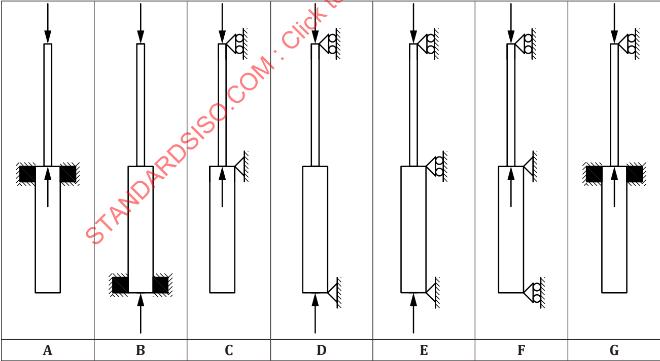
Figure A.1 — Common buckling cases for hydraulic cylinders
