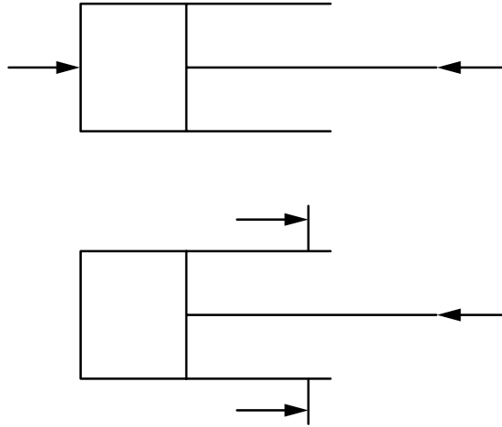
Figure 18 — Cylinder bottom, supported (upper) and unsupported (lower)
