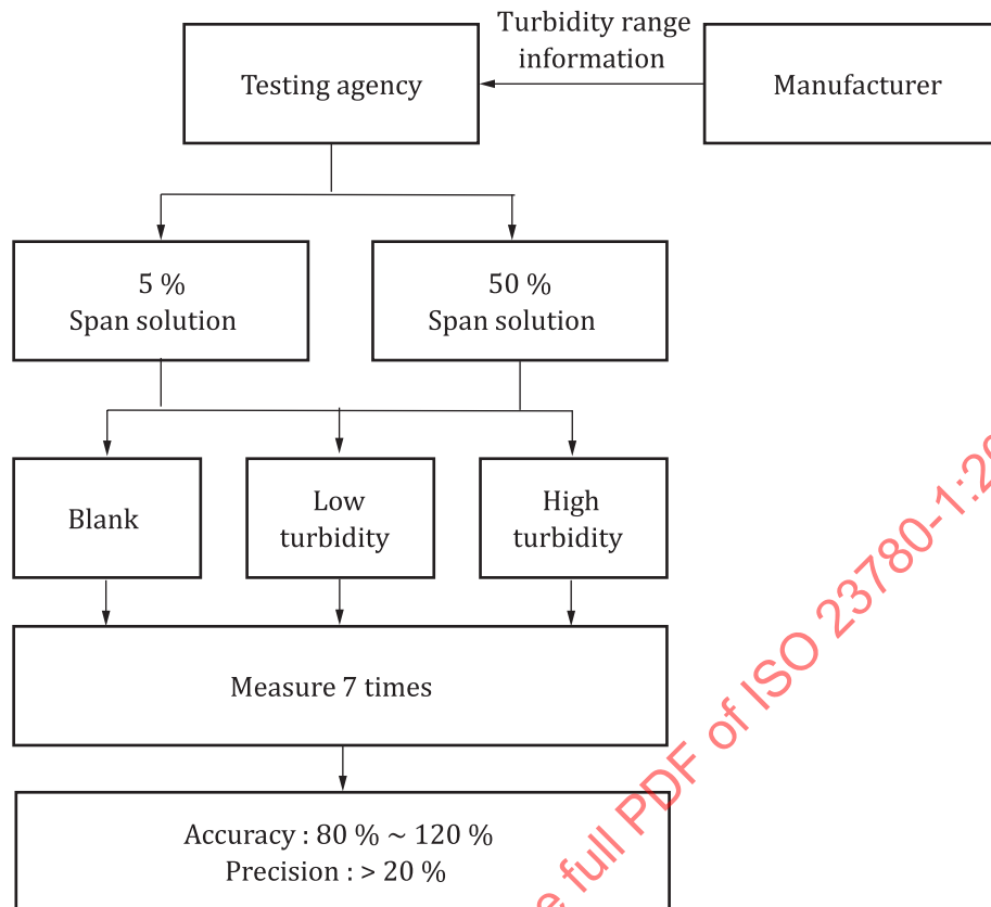
Figure 2 — Schematic of the turbidity test procedure
