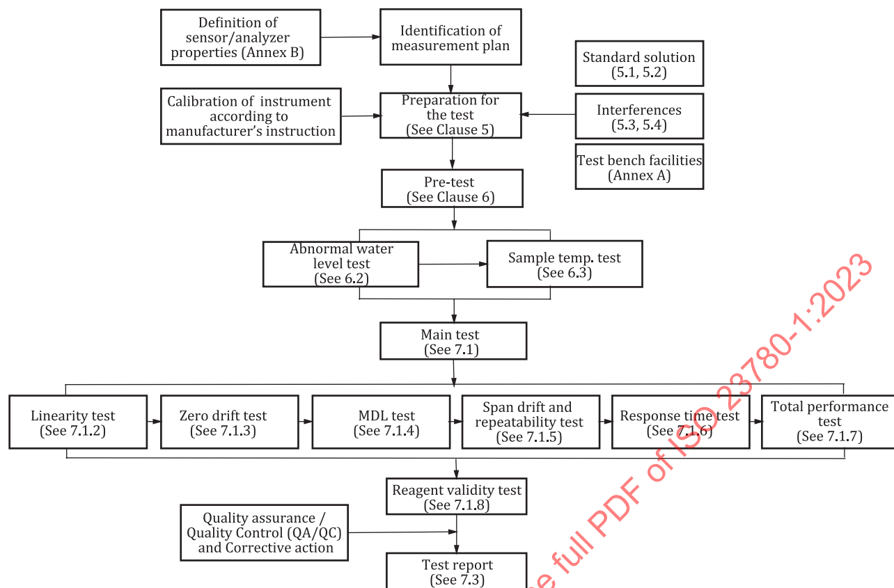
Figure 1 — Schematic of the test procedure
