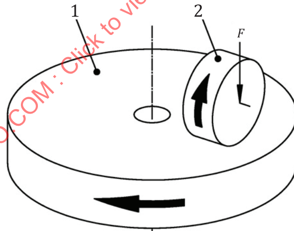
Figure 3 — Test piece and abradant in the form of wheels either of which can be driven
