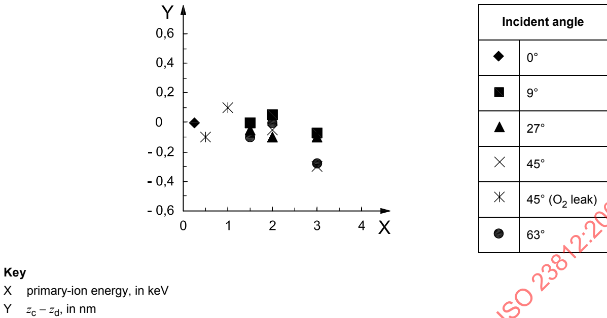
Figure B.1 — Shift of centroid positions relative to the original delta-layer position deduced using the MRI model with the same parameters for delta-layer and matrix atoms
