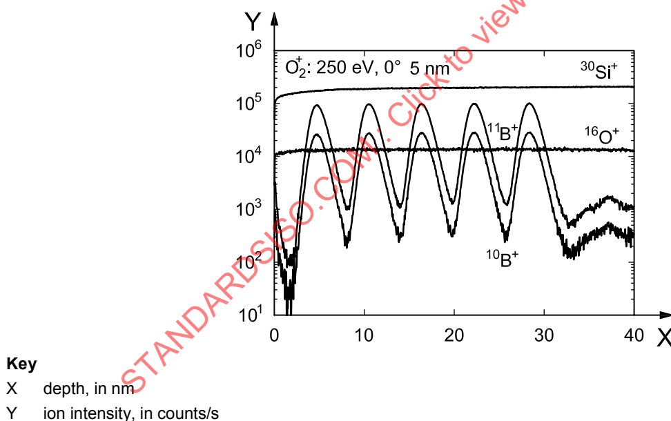
Figure 1 — SIMS depth profile of boron delta-layers in silicon [2]
