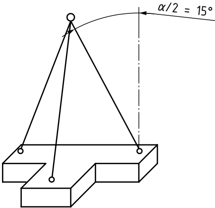
Figure A.2 — Three-legged slinging (lifting angle 30°)
