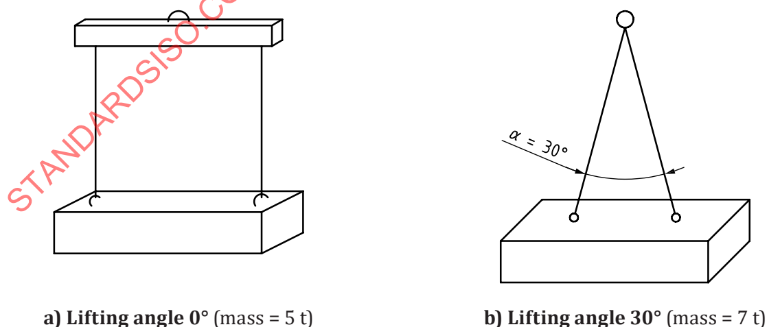
Figure A.1 — Two-legged slinging
