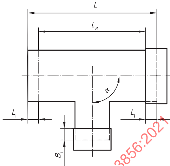
b) Unequal tee branch
