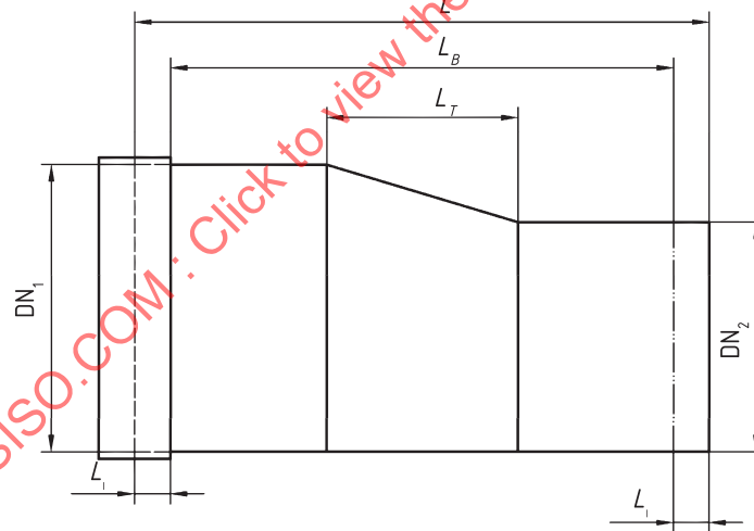
b) Eccentric reducer
